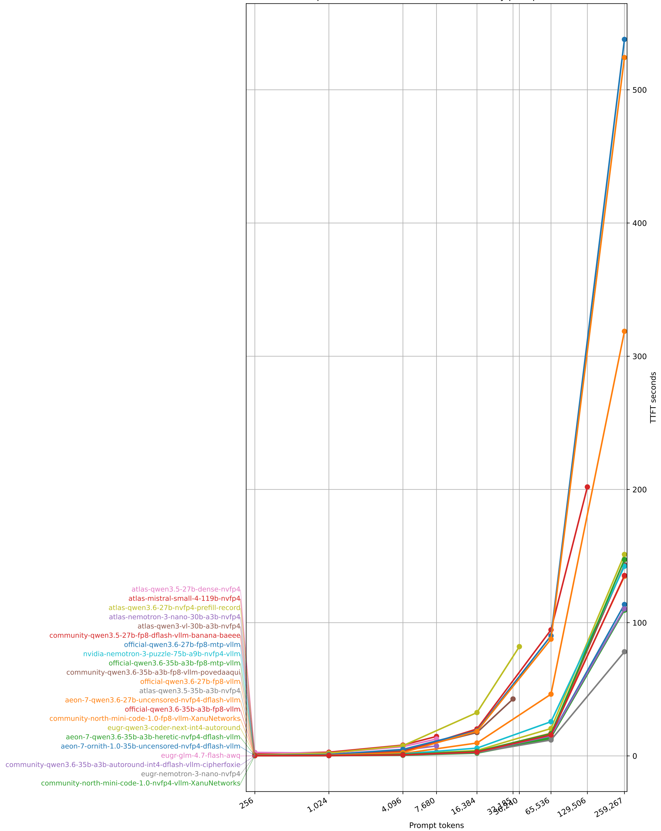
Sparkrun benchmark time to first token by prompt size
