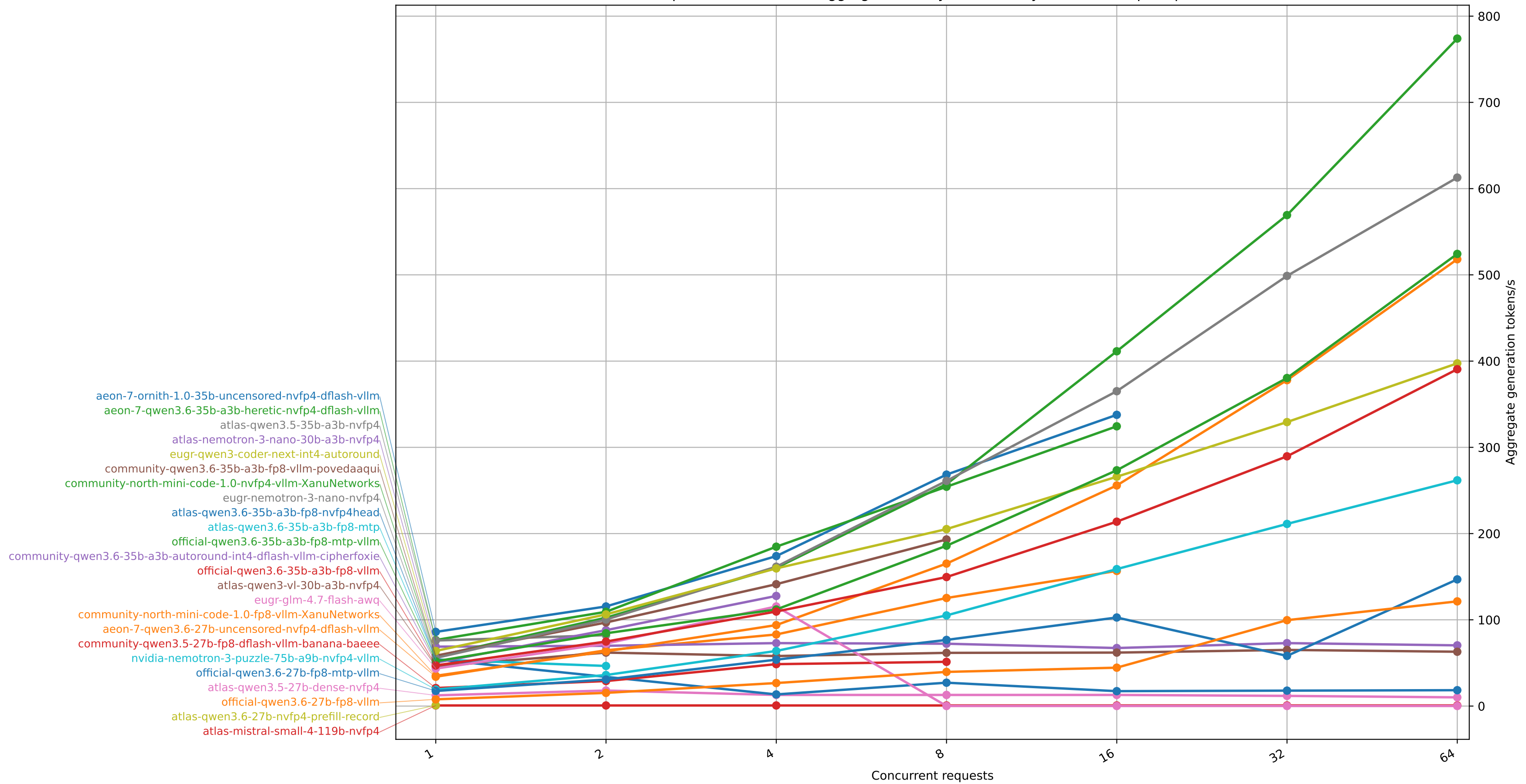
Sparkrun benchmark aggregate TPS by concurrency (1024-token prompts)
