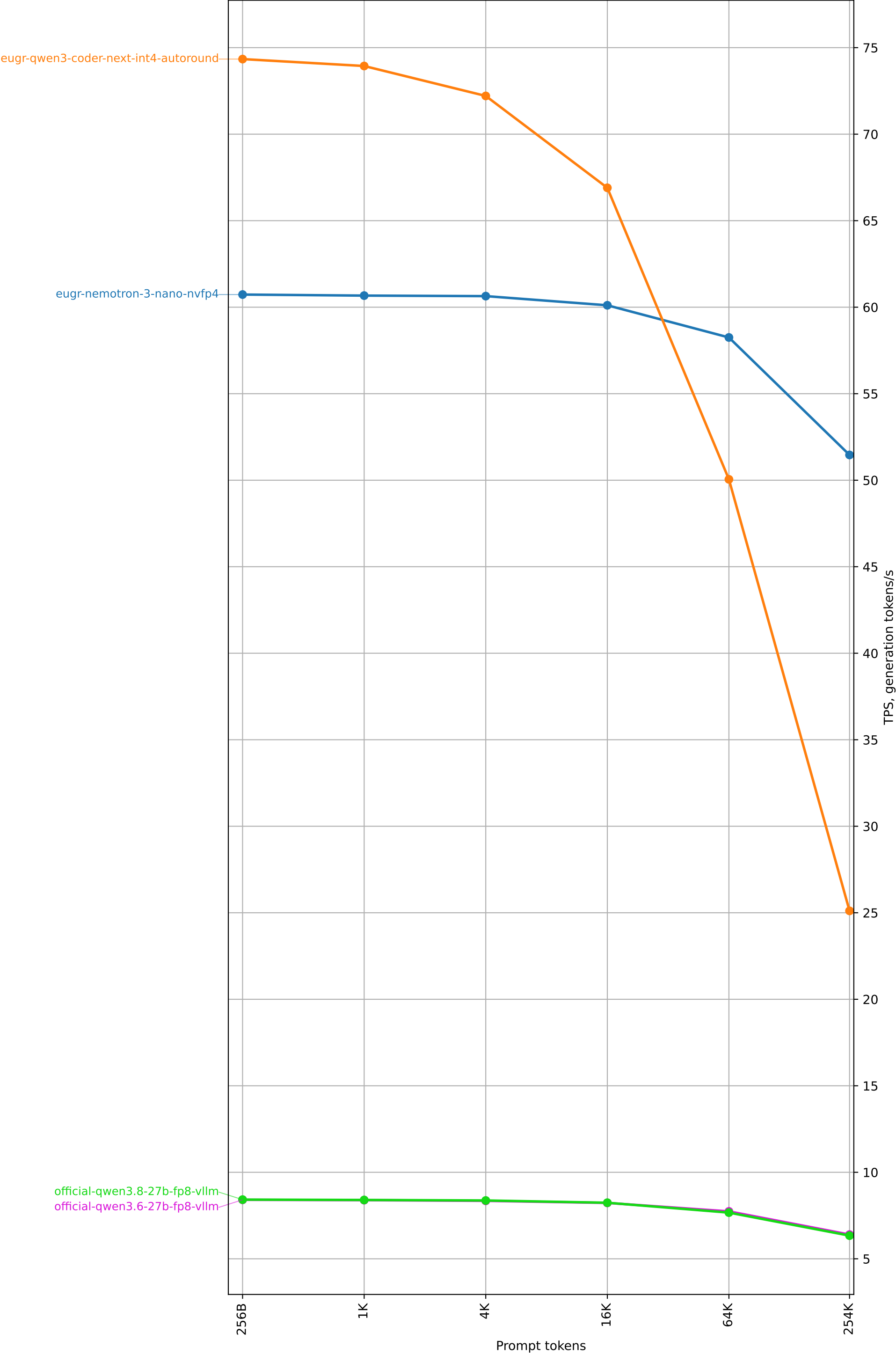
Sparkrun benchmark TPS by prompt size
