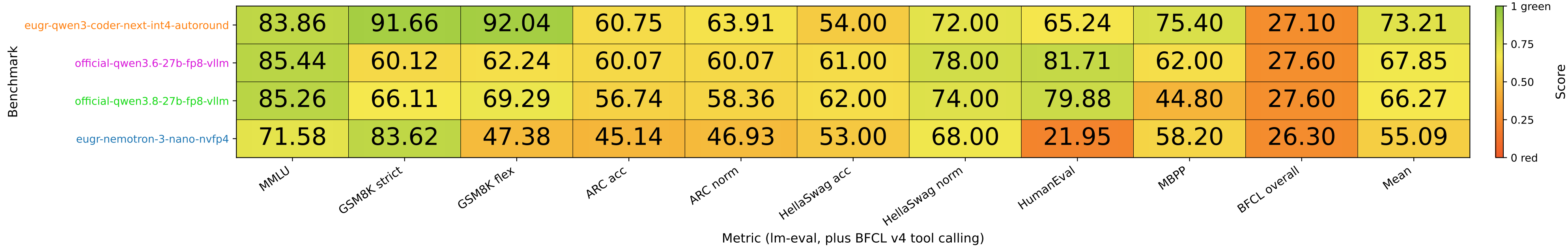
Sparkrun intelligence scores (grey = test failed or could not run)
