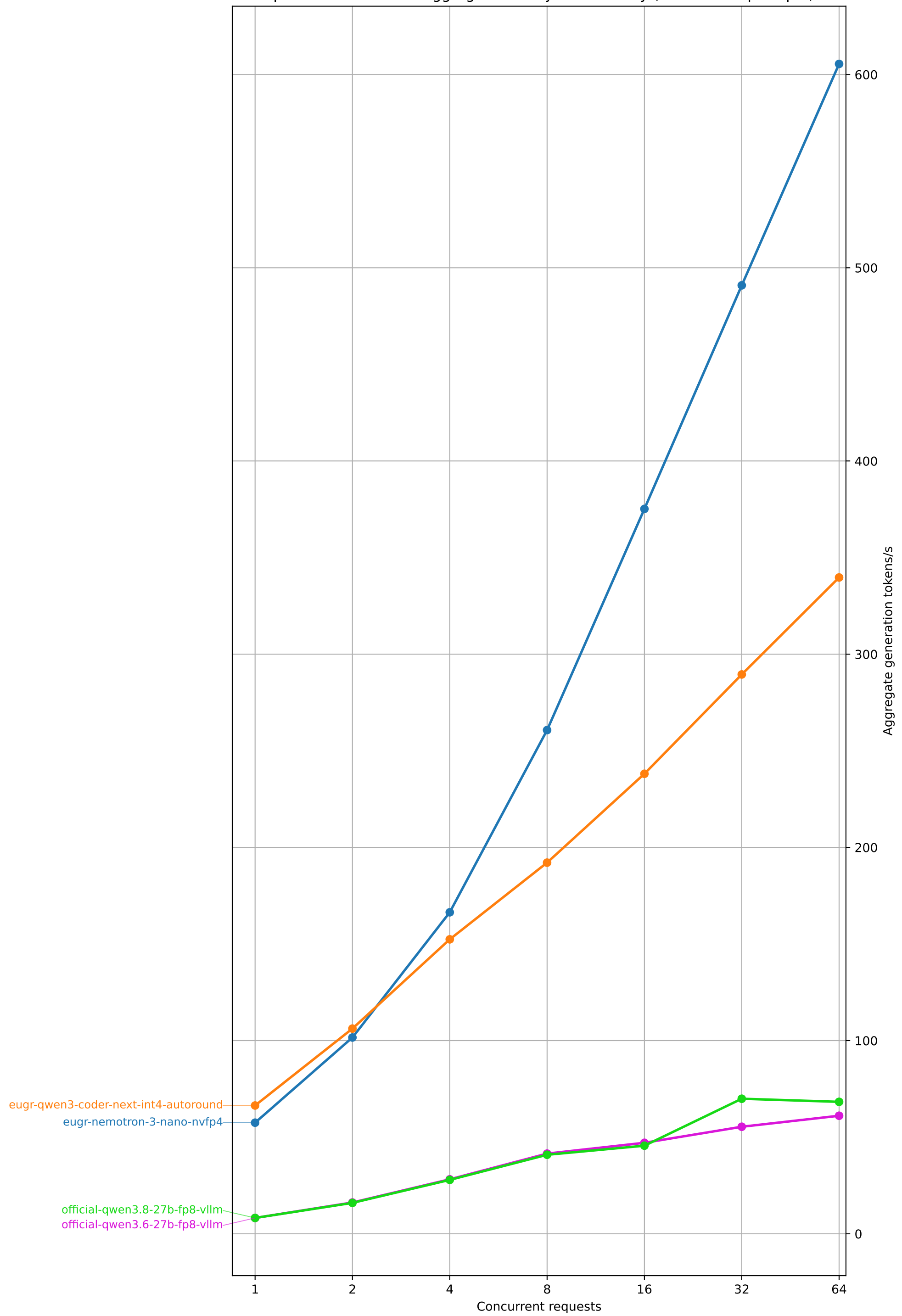
Sparkrun benchmark aggregate TPS by concurrency (1024-token prompts)
