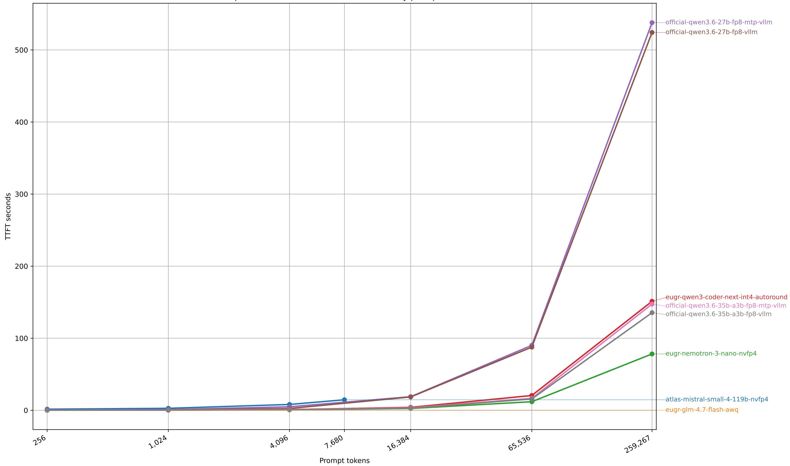
Sparkrun benchmark time to first token by prompt size
