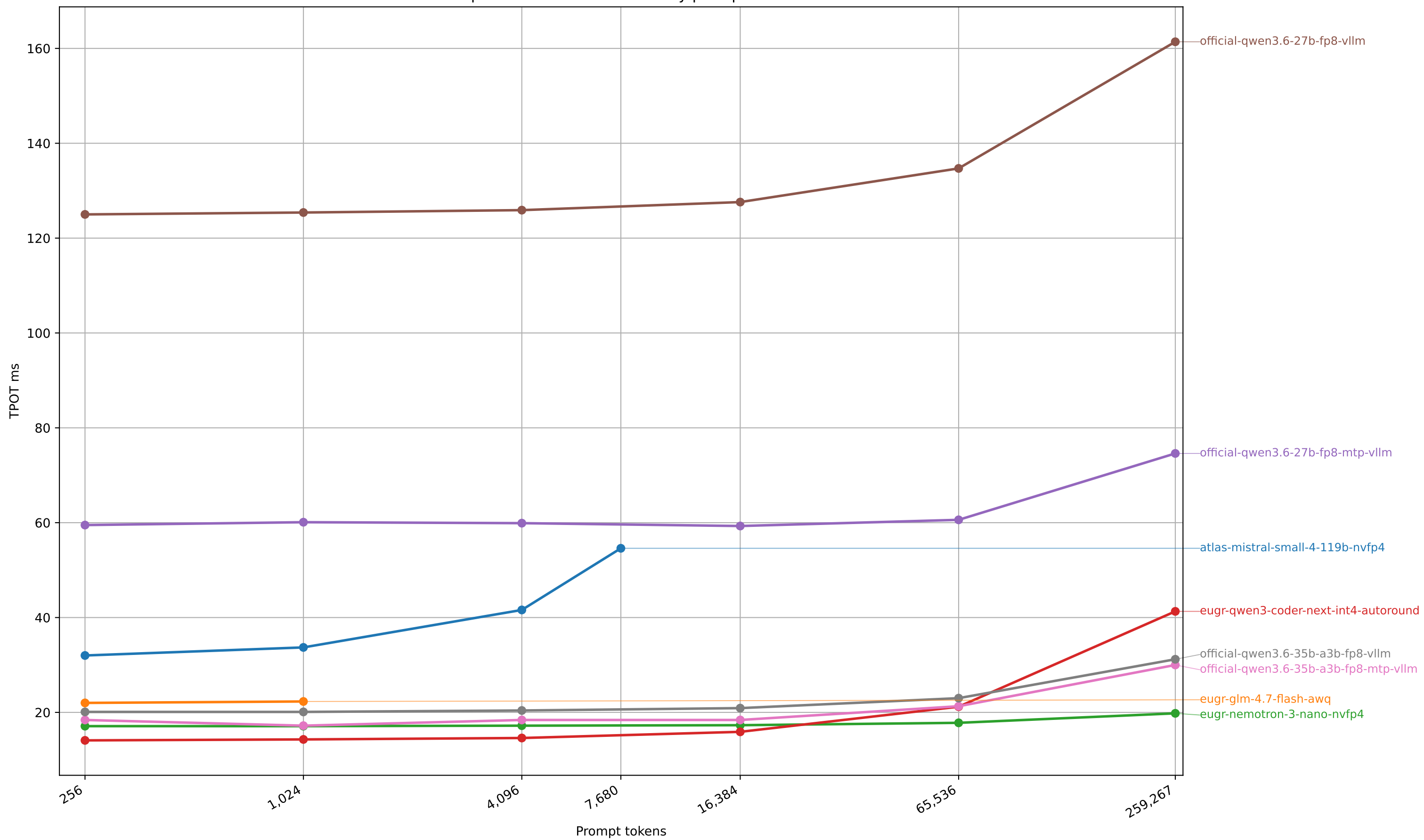
Sparkrun benchmark TPOT by prompt size
