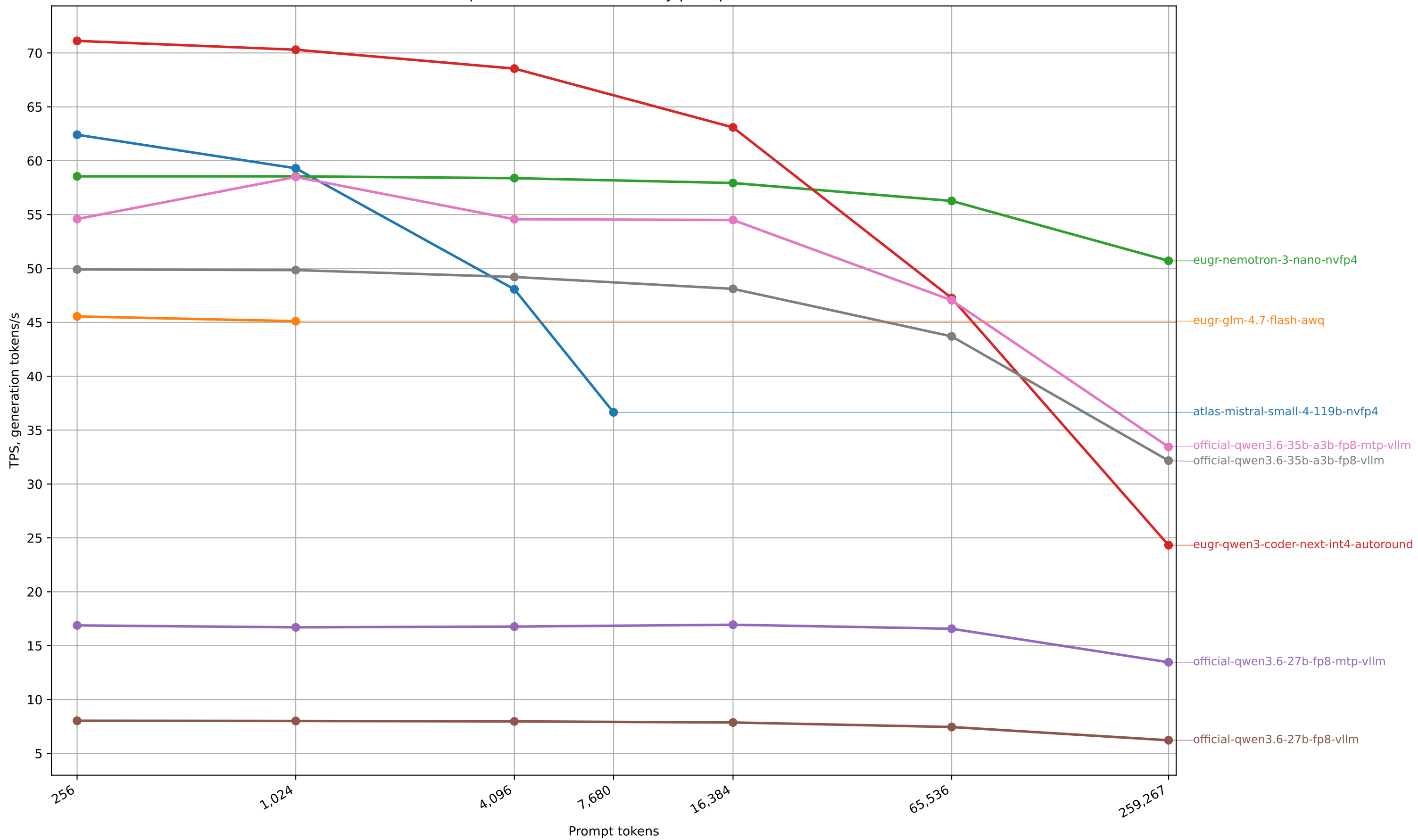
Sparkrun benchmark TPS by prompt size
