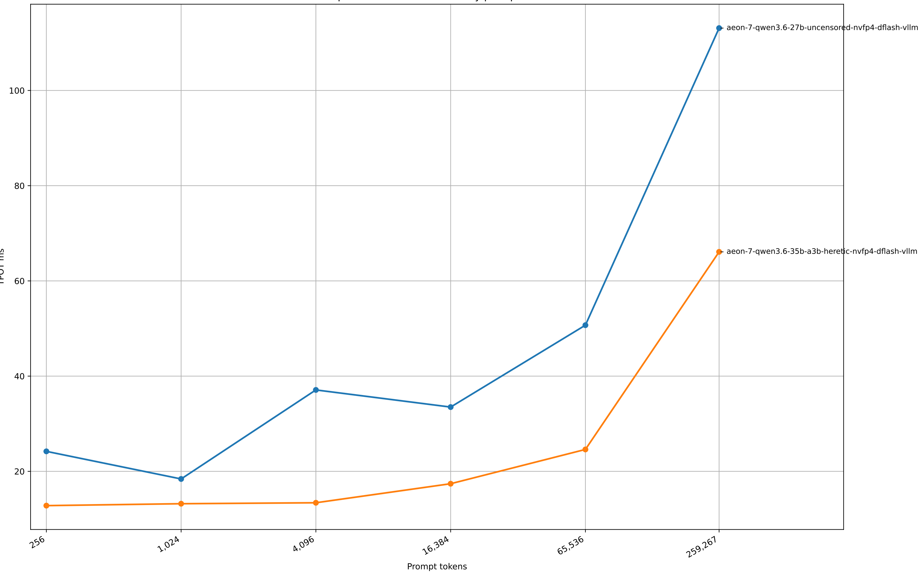
Sparkrun benchmark TPOT by prompt size
