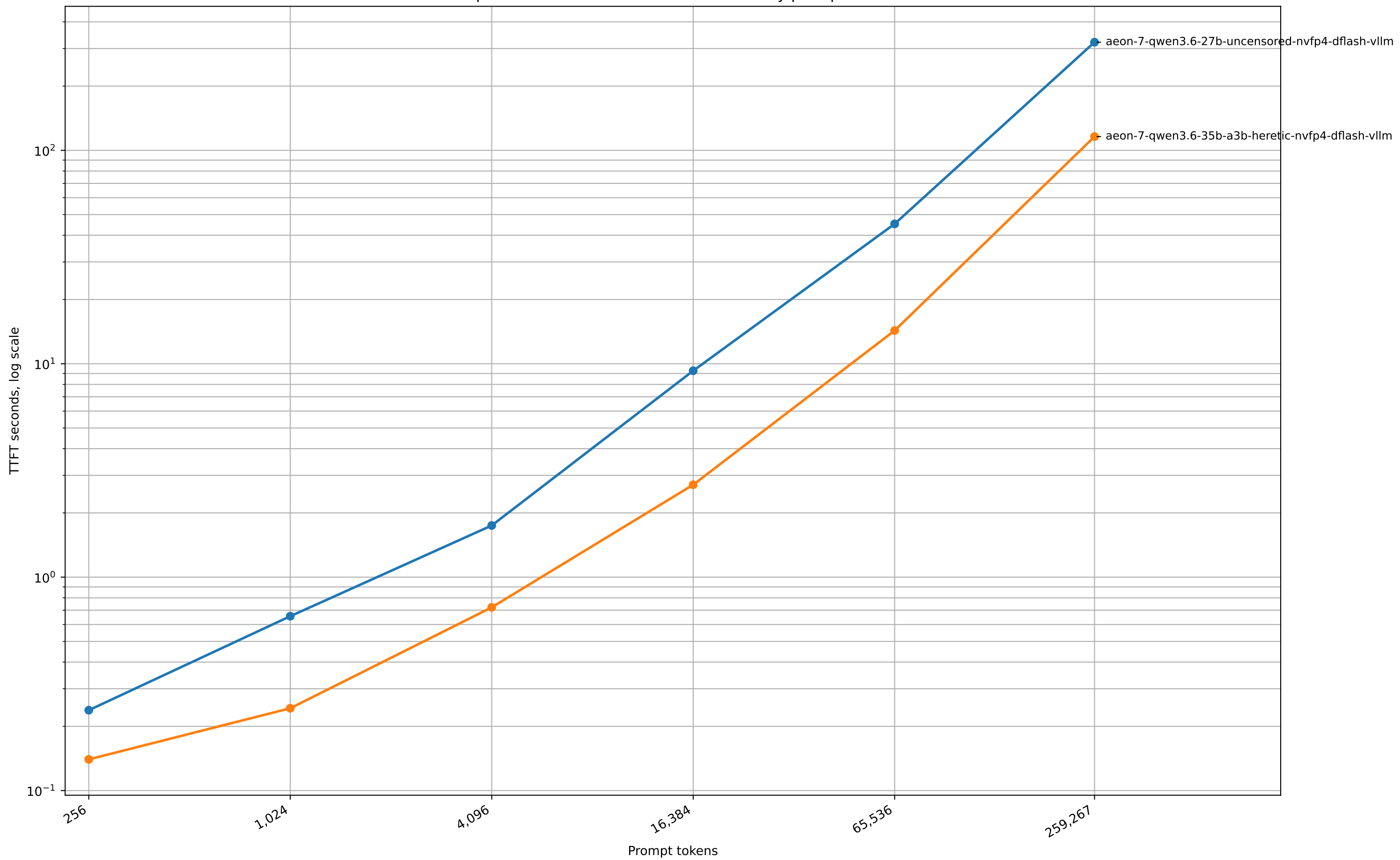
Sparkrun benchmark time to first token by prompt size
