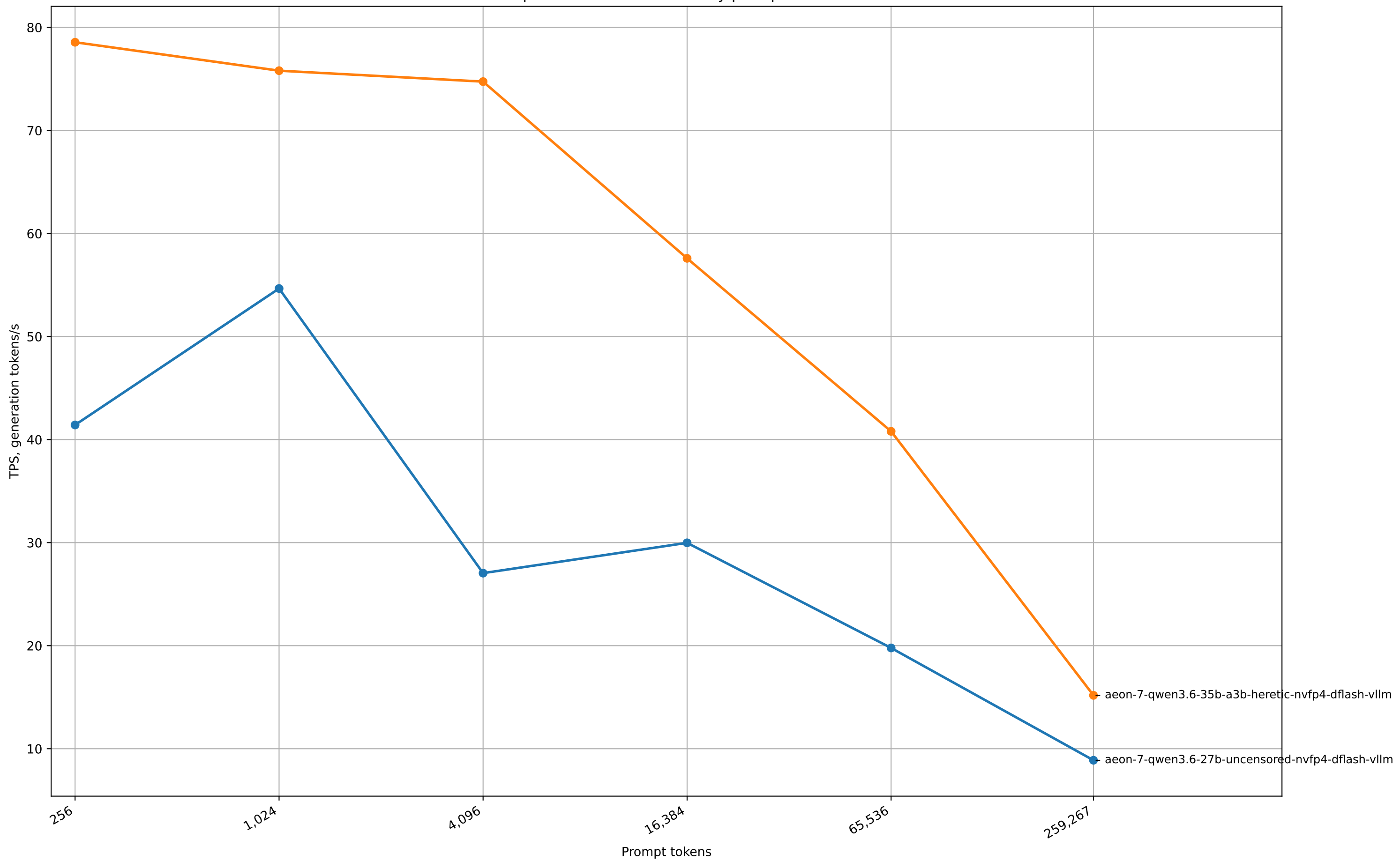
Sparkrun benchmark TPS by prompt size
