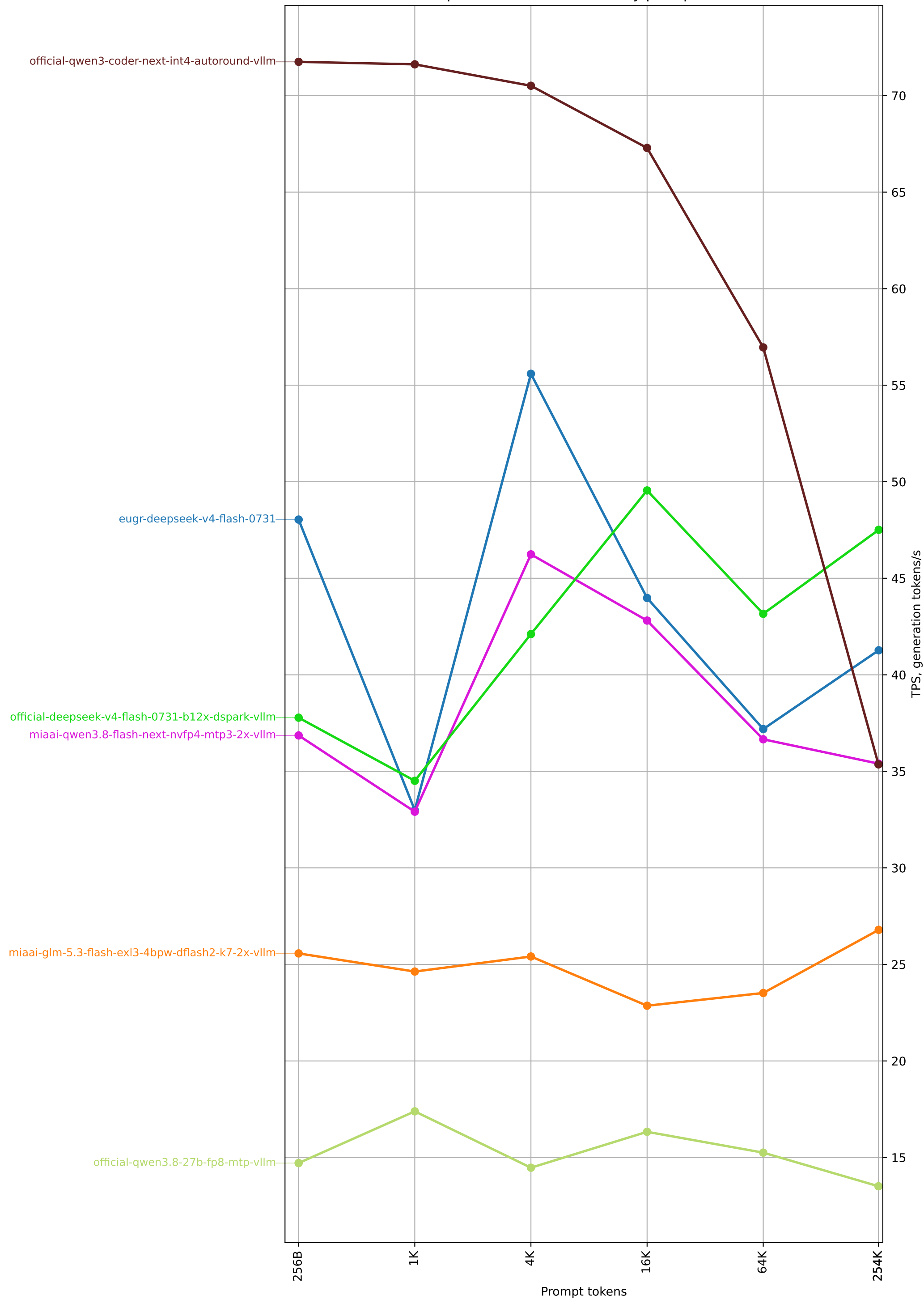
Sparkrun benchmark TPS by prompt size
