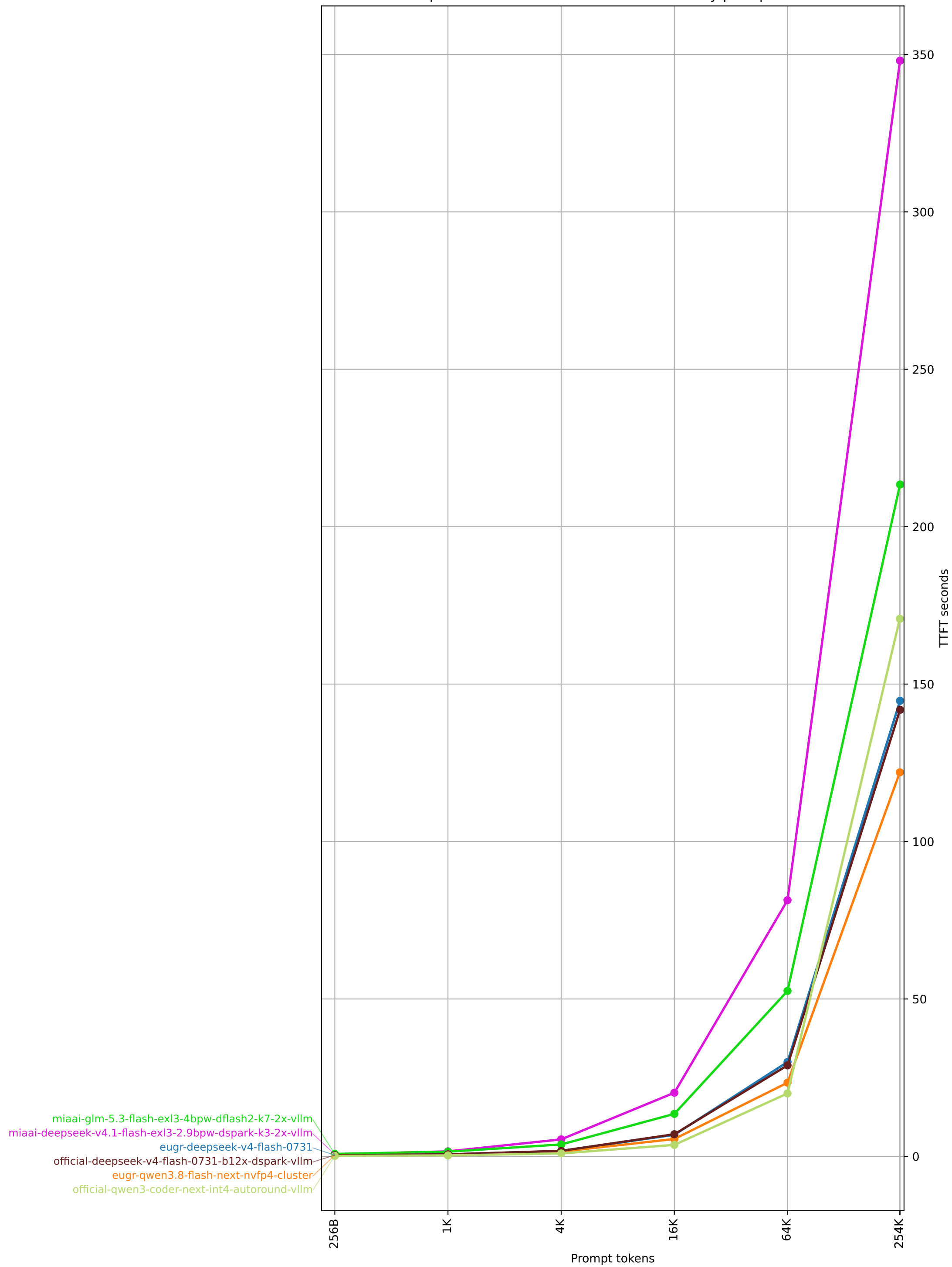
Sparkrun benchmark time to first token by prompt size
