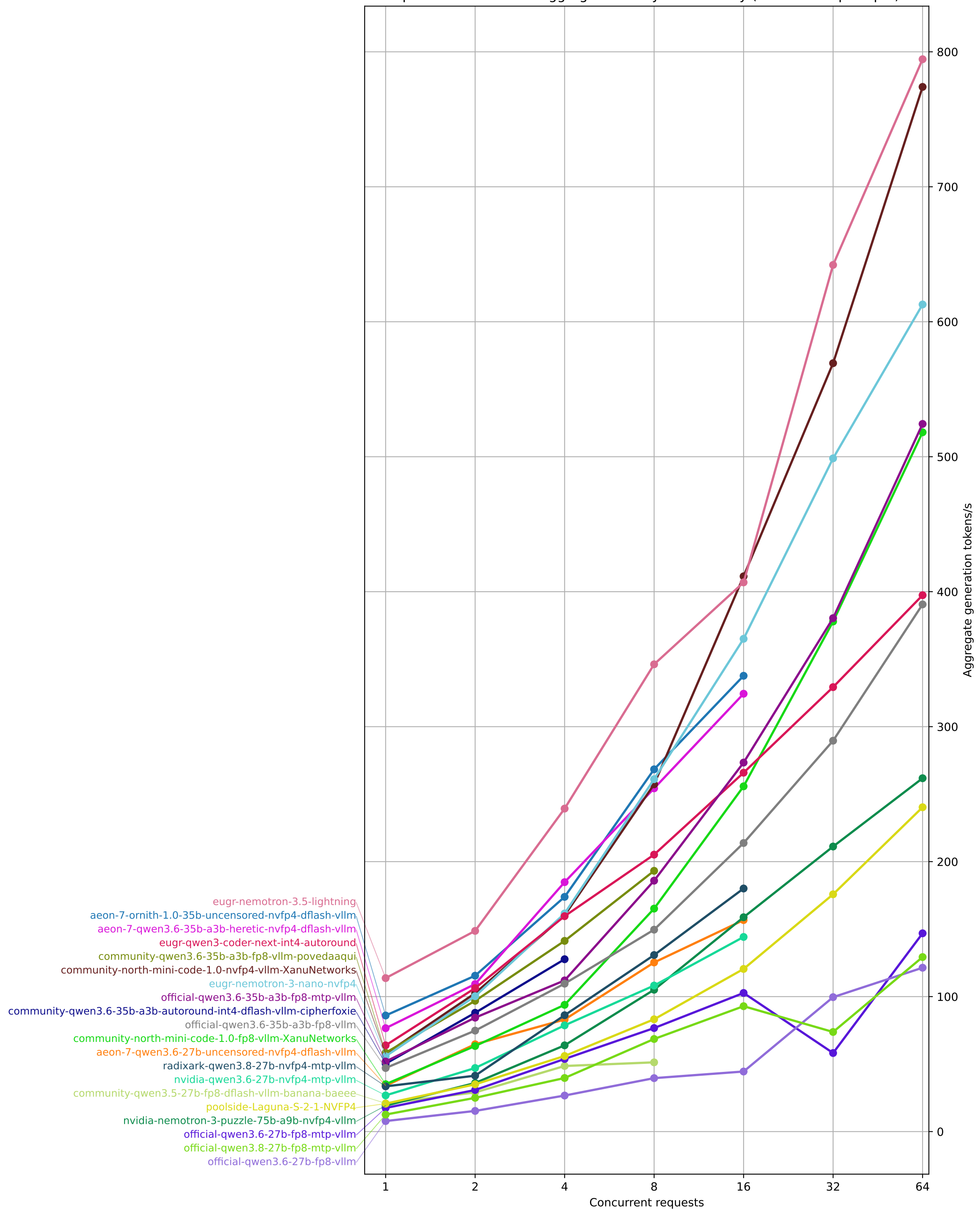
Sparkrun benchmark aggregate TPS by concurrency (1024-token prompts)
