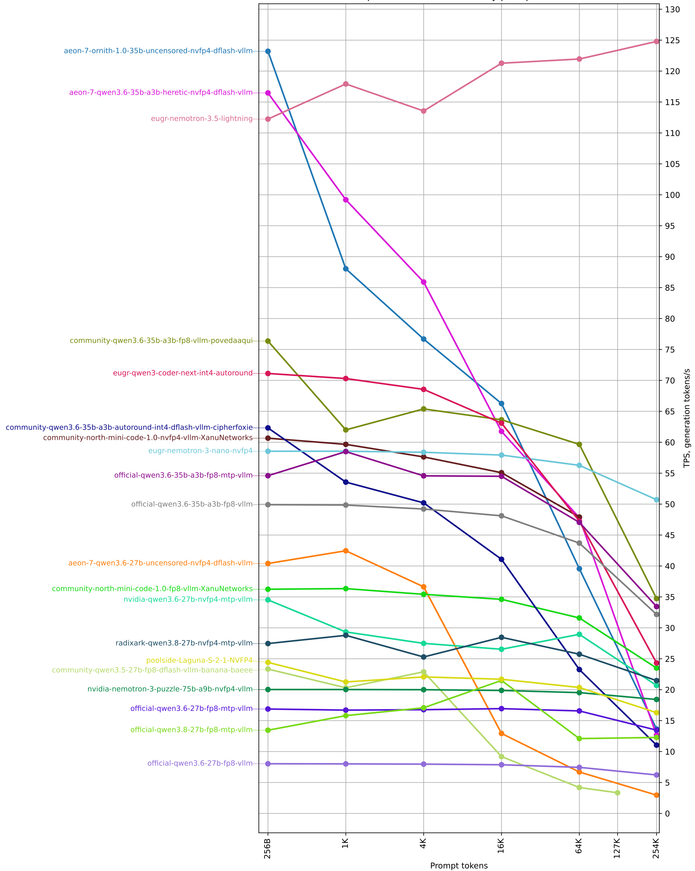
Sparkrun benchmark TPS by prompt size
