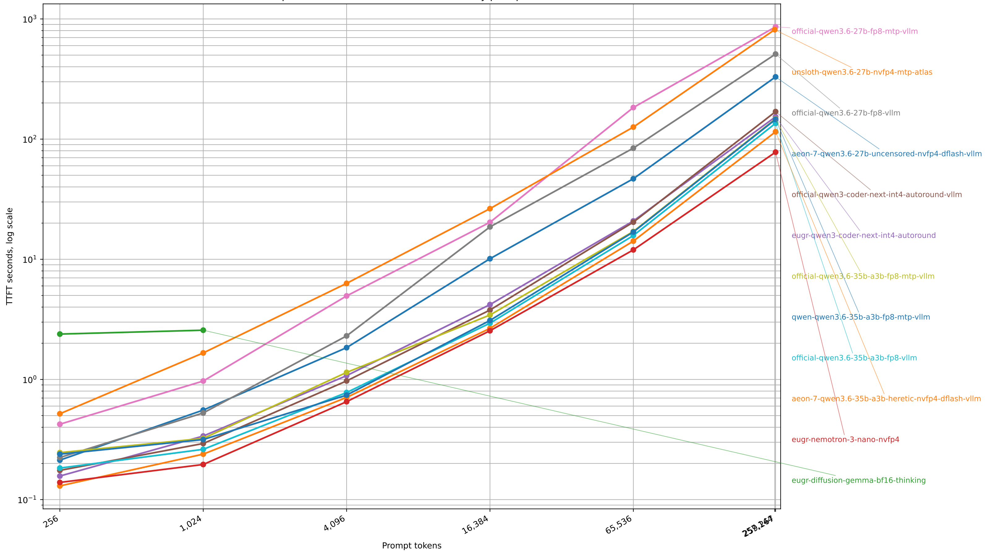
Sparkrun benchmark time to first token by prompt size
