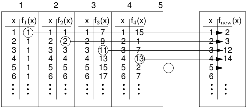
Figure 17.8 Illustration for the argument that the number of integer functions is uncountable.
