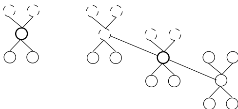
Figure 15.4 A method for finding a pivot for partitioning a list that guarantees at least a fixed fraction of the list will be in each partition. We divide the list into groups of five elements, and find the median for each group. We then recursively find the median of these n/5 medians. The median of five elements is guaranteed to have at least two in each partition. The median of three medians from a collection of 15 elements is guaranteed to have at least five elements in each partition.
