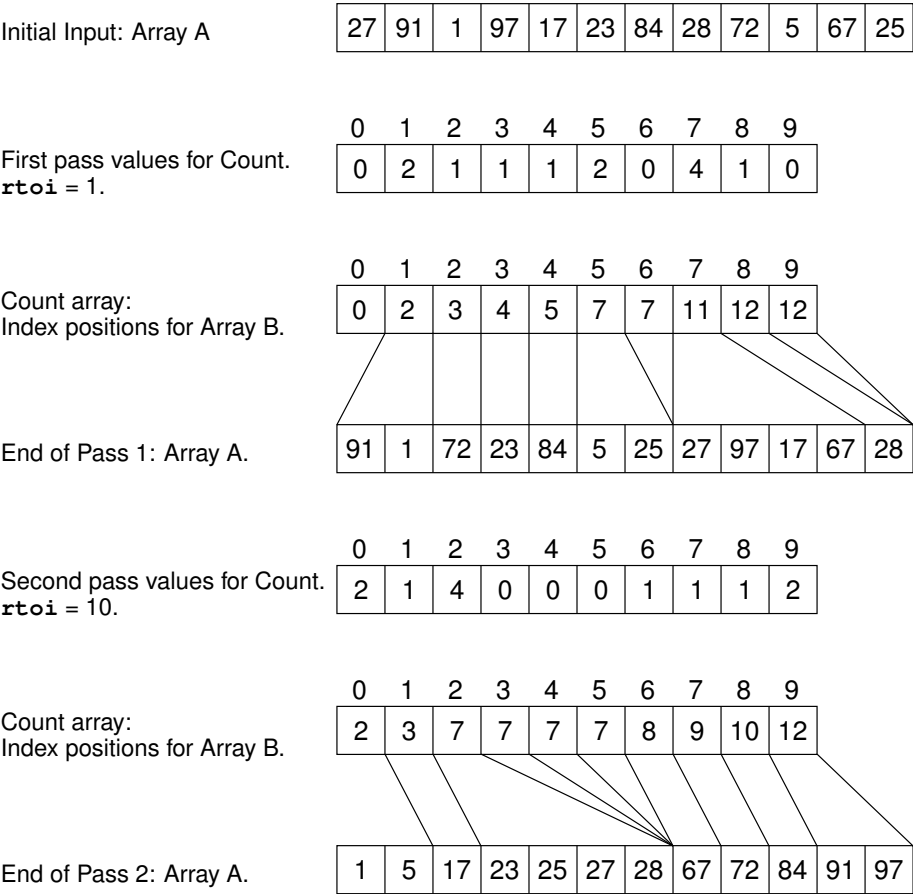
Figure 7.12 An example showing function radix applied to the input of Figure 7.11. Row 1 shows the initial values within the input array. Row 2 shows the values for array cnt after counting the number of records for each bin. Row 3 shows the index values stored in array cnt . For example, cnt [0] is 0, indicating no input values are in bin 0. Cnt [1] is 2, indicating that array B positions 0 and 1 will hold the values for bin 1. Cnt [2] is 3, indicating that array B position 2 will hold the (single) value for bin 2. Cnt [7] is 11, indicating that array B positions 7 through 10 will hold the four values for bin 7. Row 4 shows the results of the first pass of the Radix Sort. Rows 5 through 7 show the equivalent steps for the second pass.
