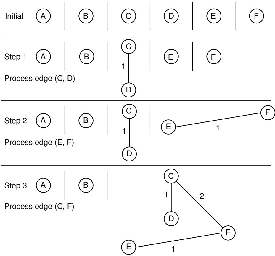
Figure 11.23 Illustration of the first three steps of Kruskal’s MST algorithm as applied to the graph of Figure 11.19.
