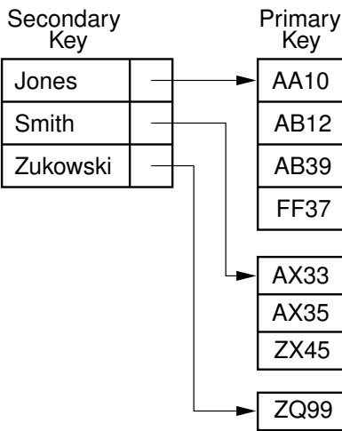
Figure 10.4 Illustration of an inverted list. Each secondary key value is stored in the secondary key list. Each secondary key value on the list has a pointer to a list of the primary keys whose associated records have that secondary key value.
