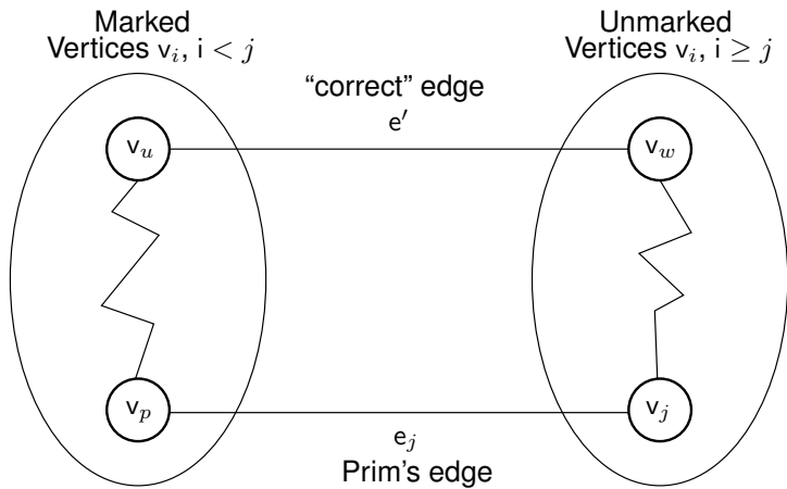
Figure 11.22 Prim’s MST algorithm proof. The left oval contains that portion of the graph where Prim’s MST and the “true” MST \mathbf{T} agree. The right oval contains the rest of the graph. The two portions of the graph are connected by (at least) edges e_j (selected by Prim’s algorithm to be in the MST) and e' (the “correct” edge to be placed in the MST). Note that the path from v_w to v_j cannot include any marked vertex v_i, i \leq j , because to do so would form a cycle.
