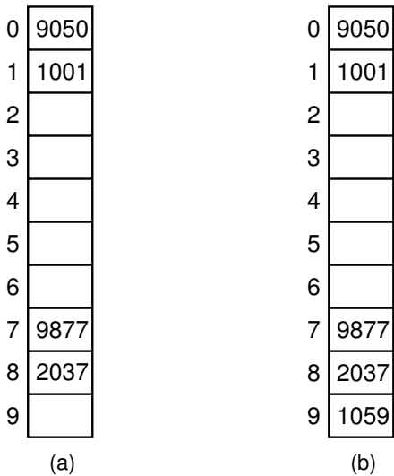
Figure 9.6 Example of problems with linear probing. (a) Four values are inserted in the order 1001, 9050, 9877, and 2037 using hash function h(K) = K \bmod 10 . (b) The value 1059 is added to the hash table.
