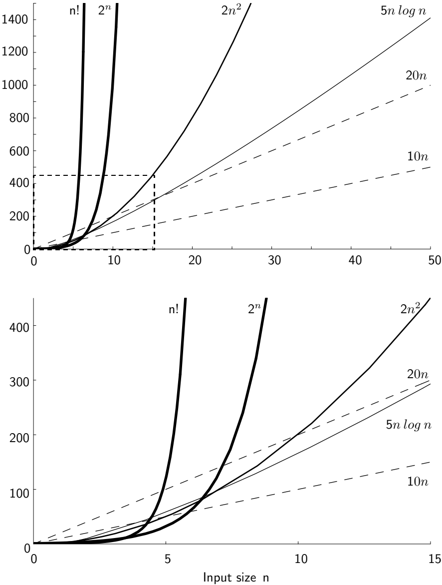
Figure 3.1 Two views of a graph illustrating the growth rates for six equations. The bottom view shows in detail the lower-left portion of the top view. The horizontal axis represents input size. The vertical axis can represent time, space, or any other measure of cost.
