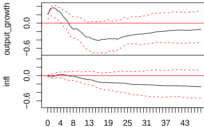
SVAR Impulse Response from romer_inv (cumulative)
