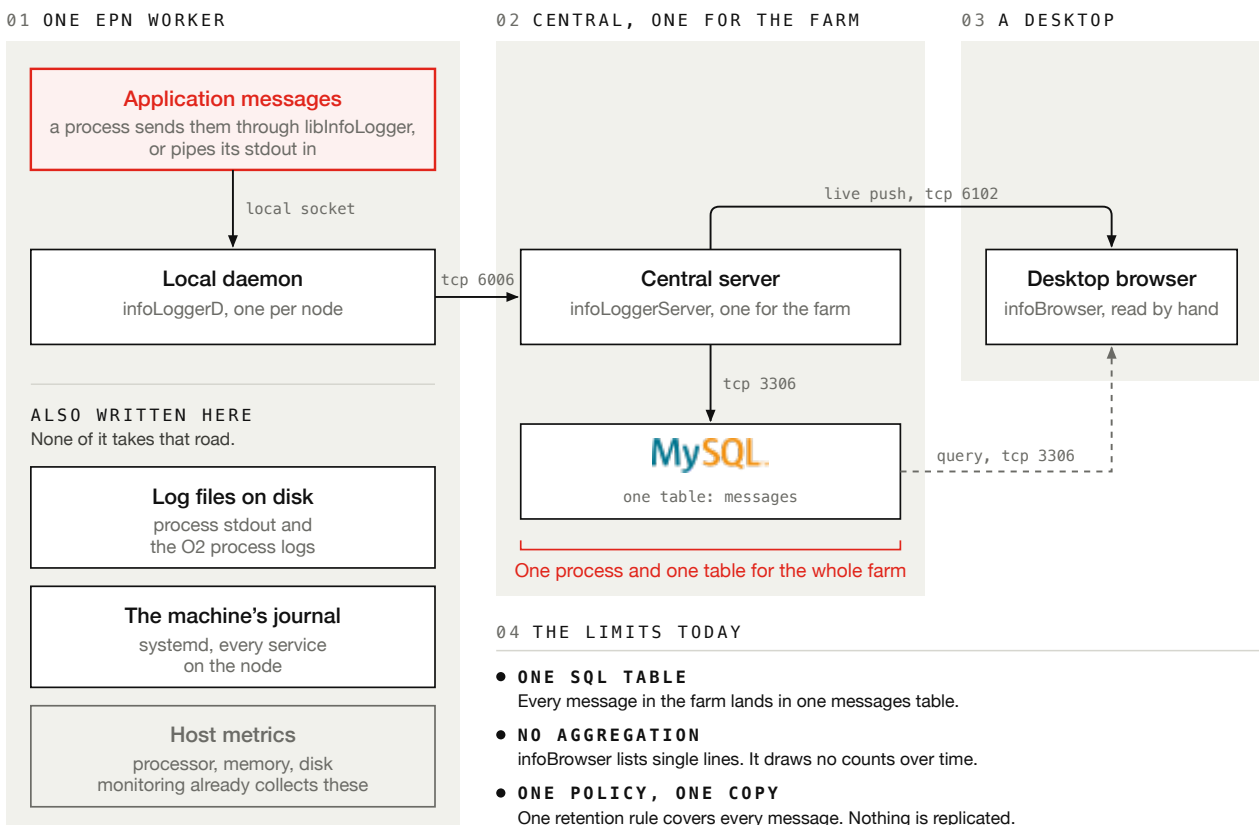
Figure 1: InfoLogger carries only what a process sends it, and the process logs on disk and the journal never take that road.
