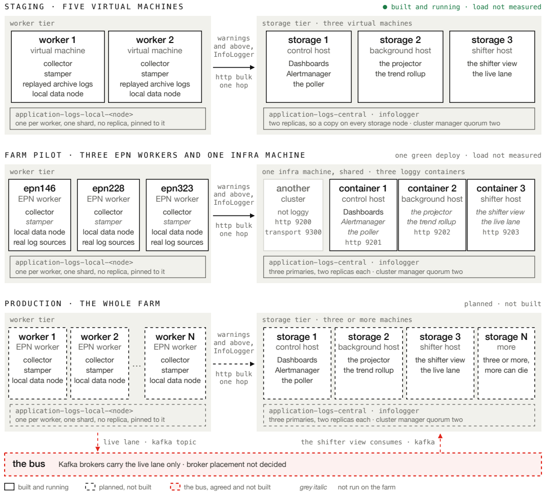
Figure 7: Staging and the farm pilot exist, and production is the same design with a bus and a bigger storage tier.
