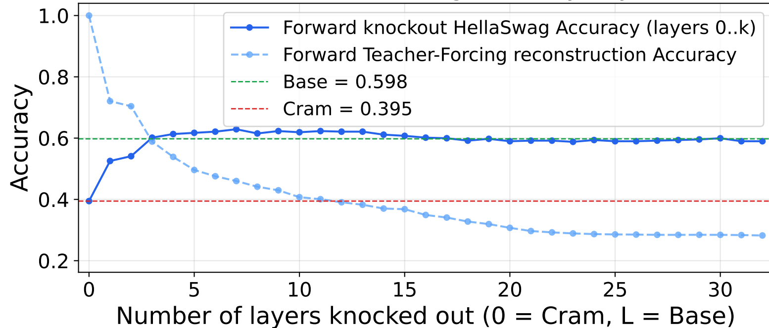
Forward knockout HellaSwag Accuracy (layers 0..k)
