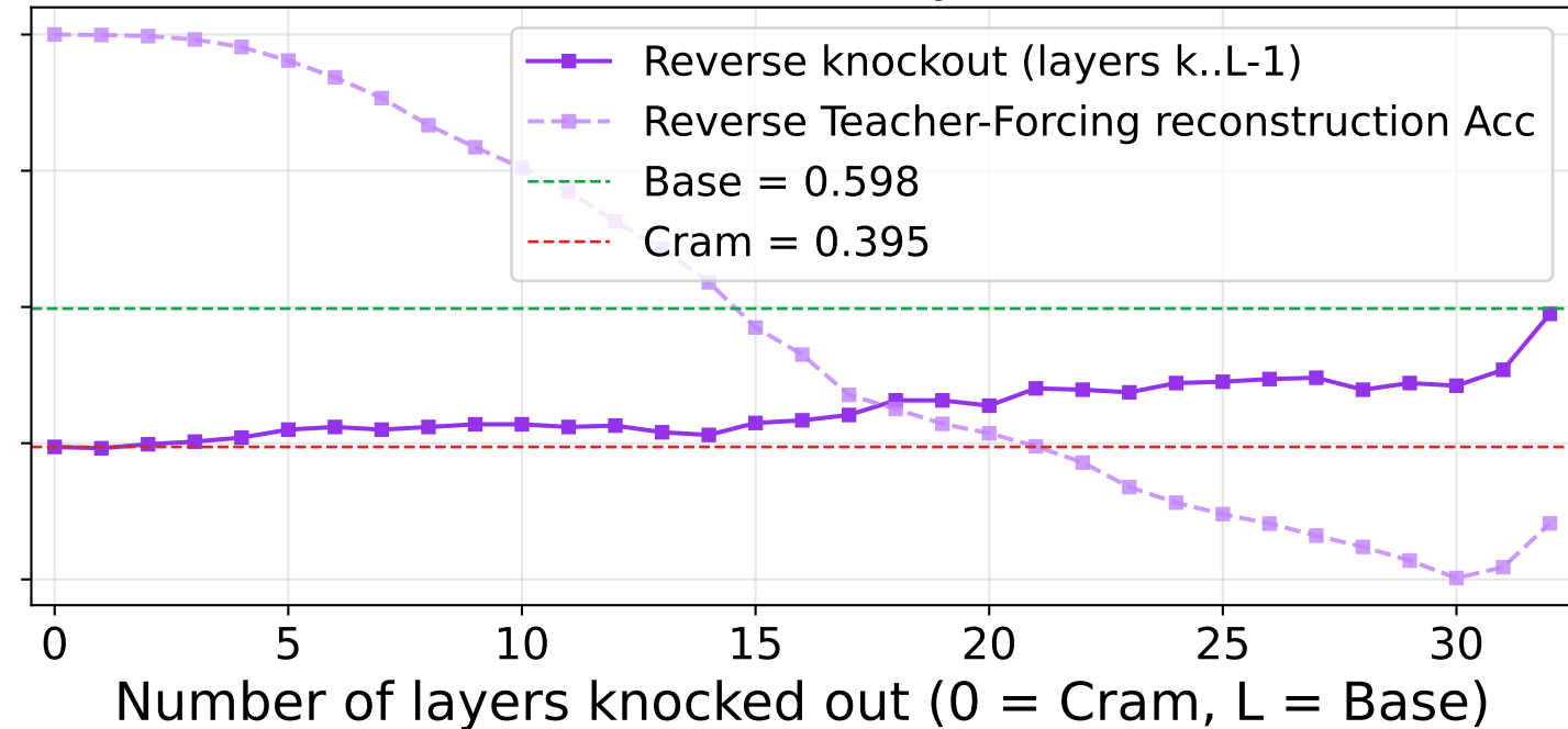
Reverse knockout (layers k..L-1)
