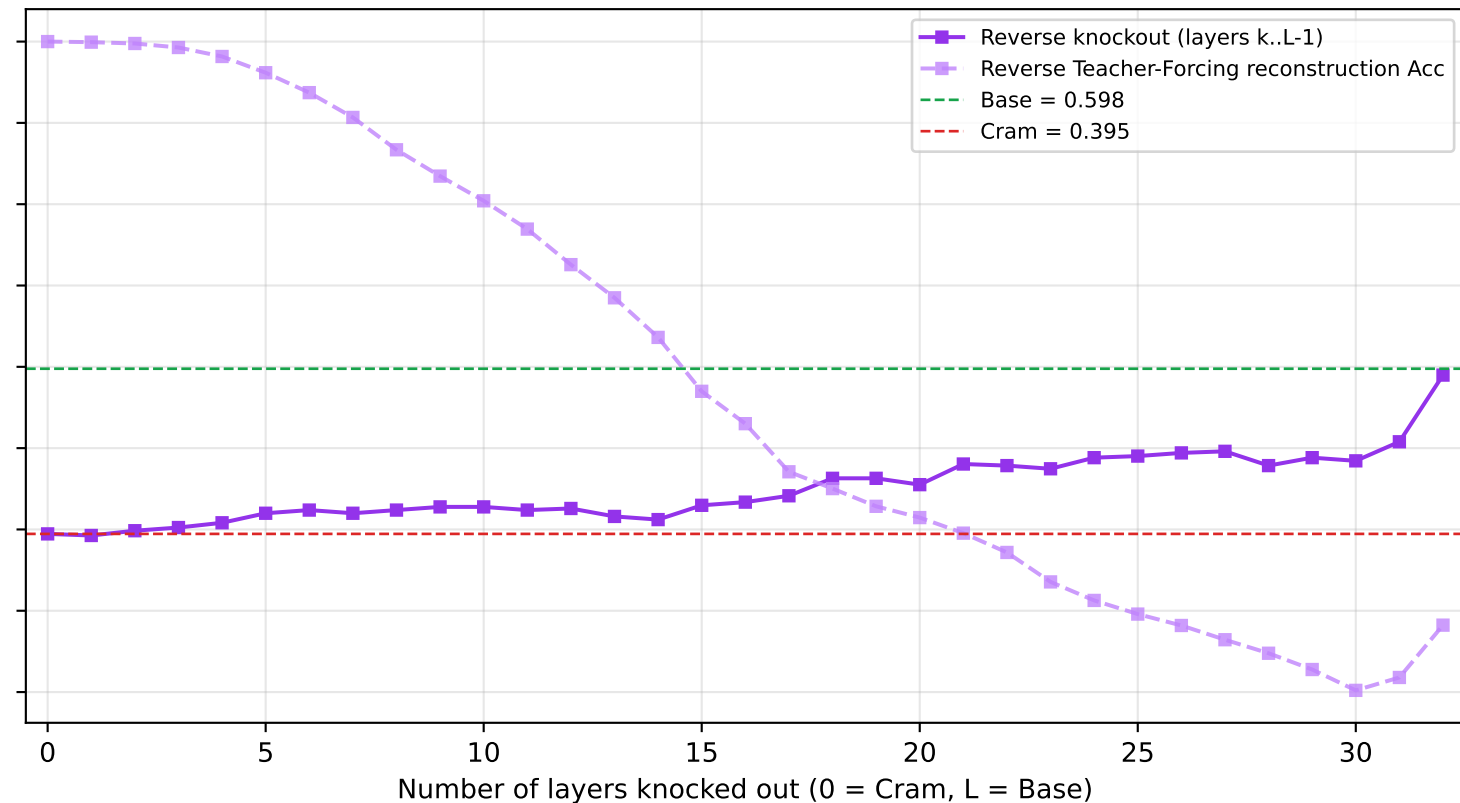
Reverse knockout (layers k..L-1)
