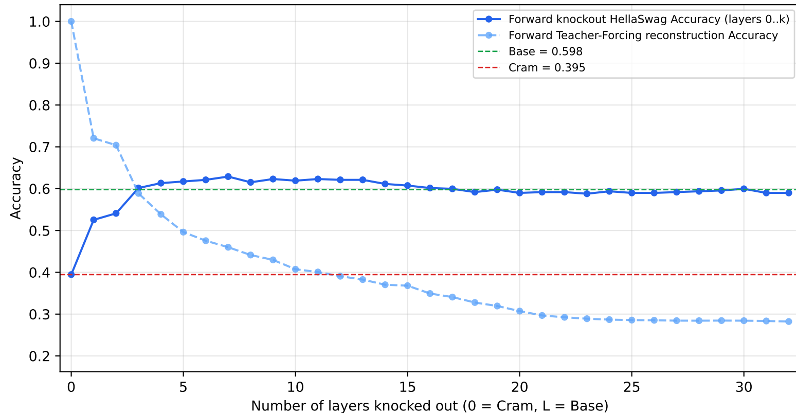
Forward knockout HellaSwag Accuracy (layers 0..k)
