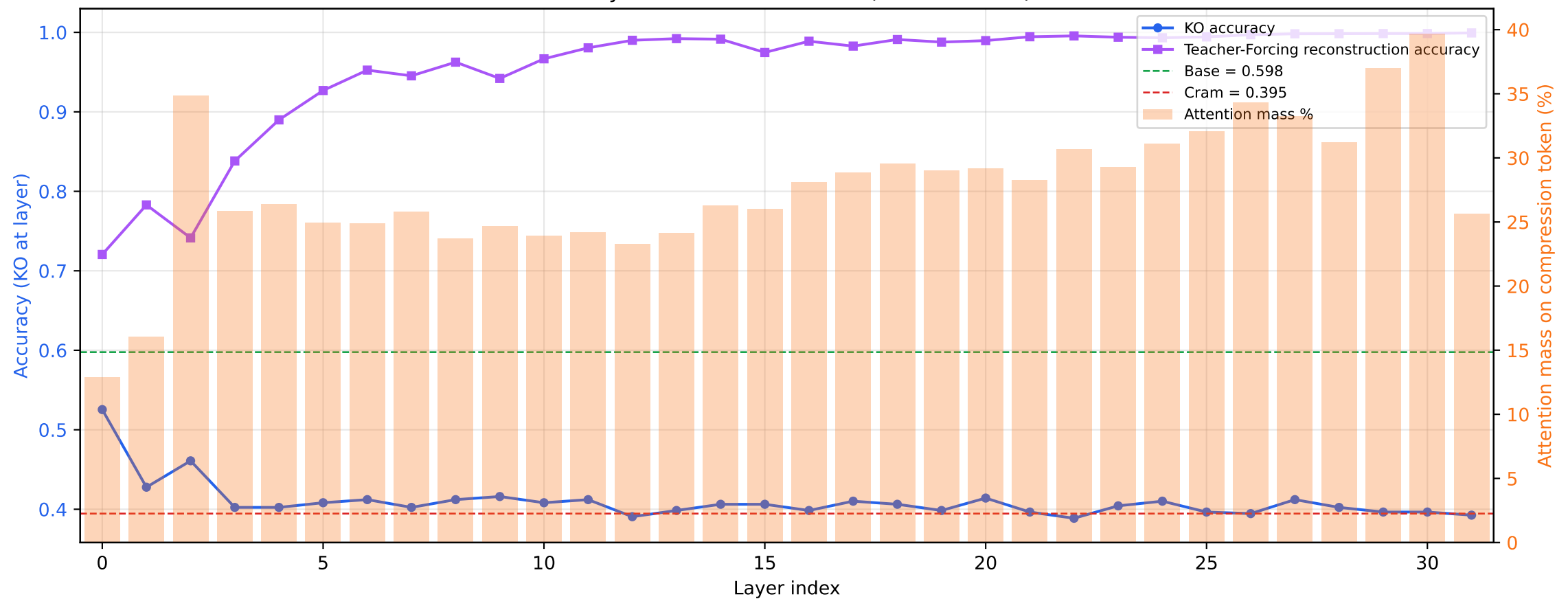
Per-Layer Attention Knockout (Llama-3.1-8B)
