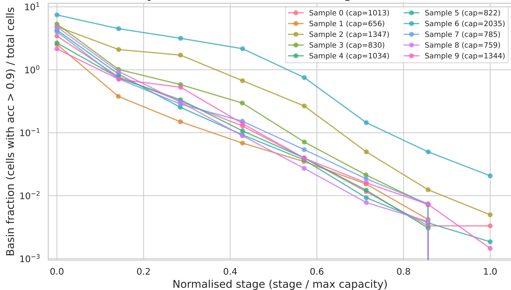
Accuracy basin size vs. normalised stage — Llama-3.1-8B
