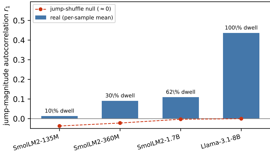
Dwell-and-jump basin structure emerges with scale
