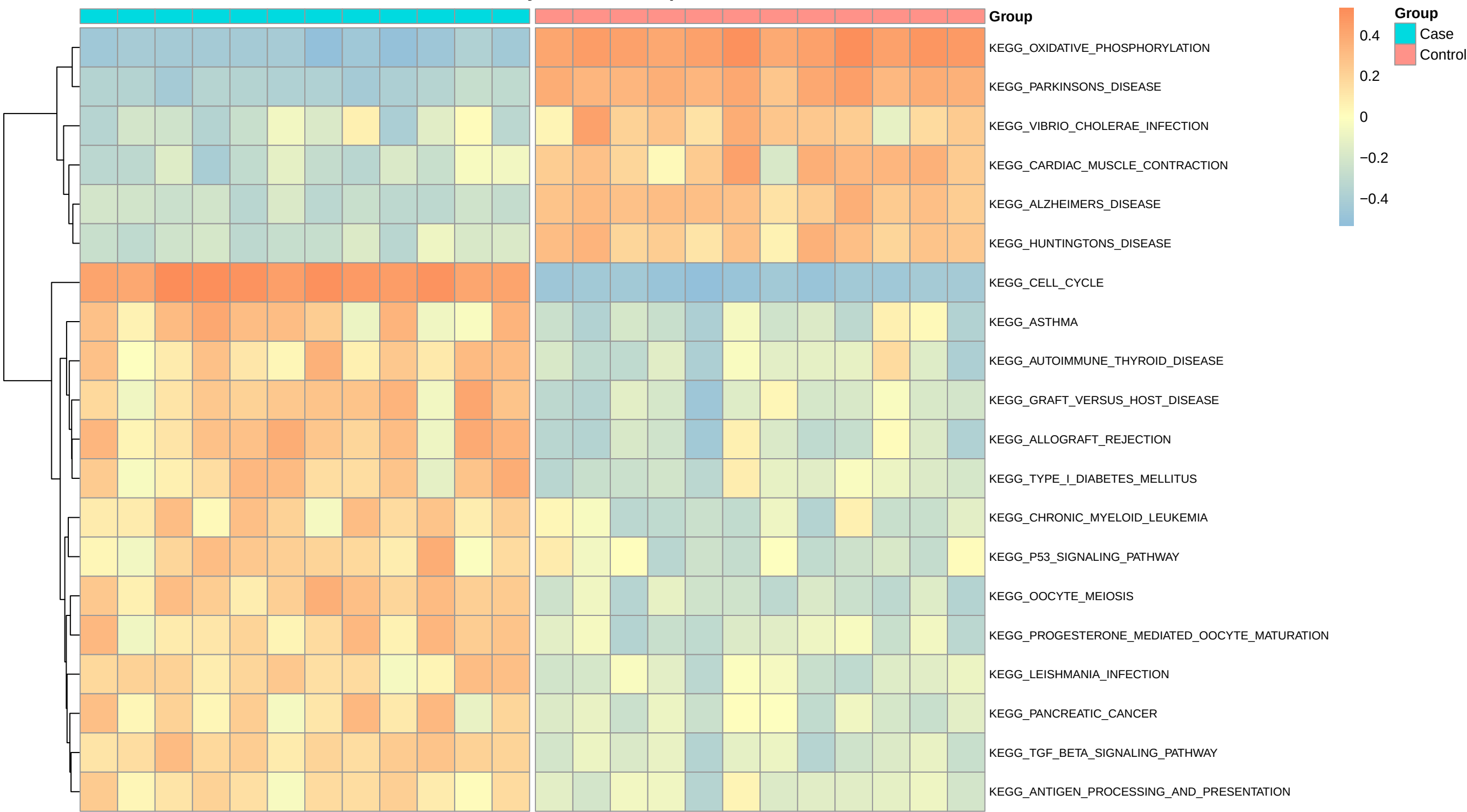
Immune Pathway GSVA Heatmap
