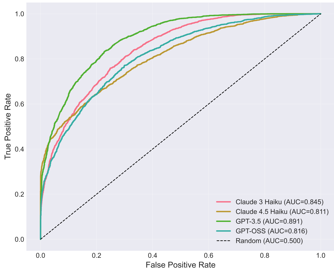
Class-Level Detection Performance
