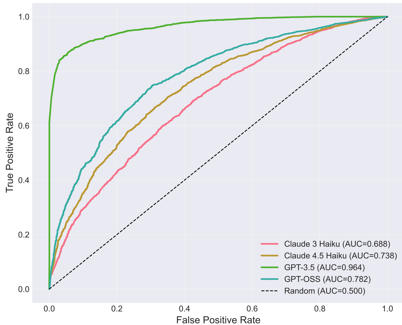
Function-Level Detection Performance
