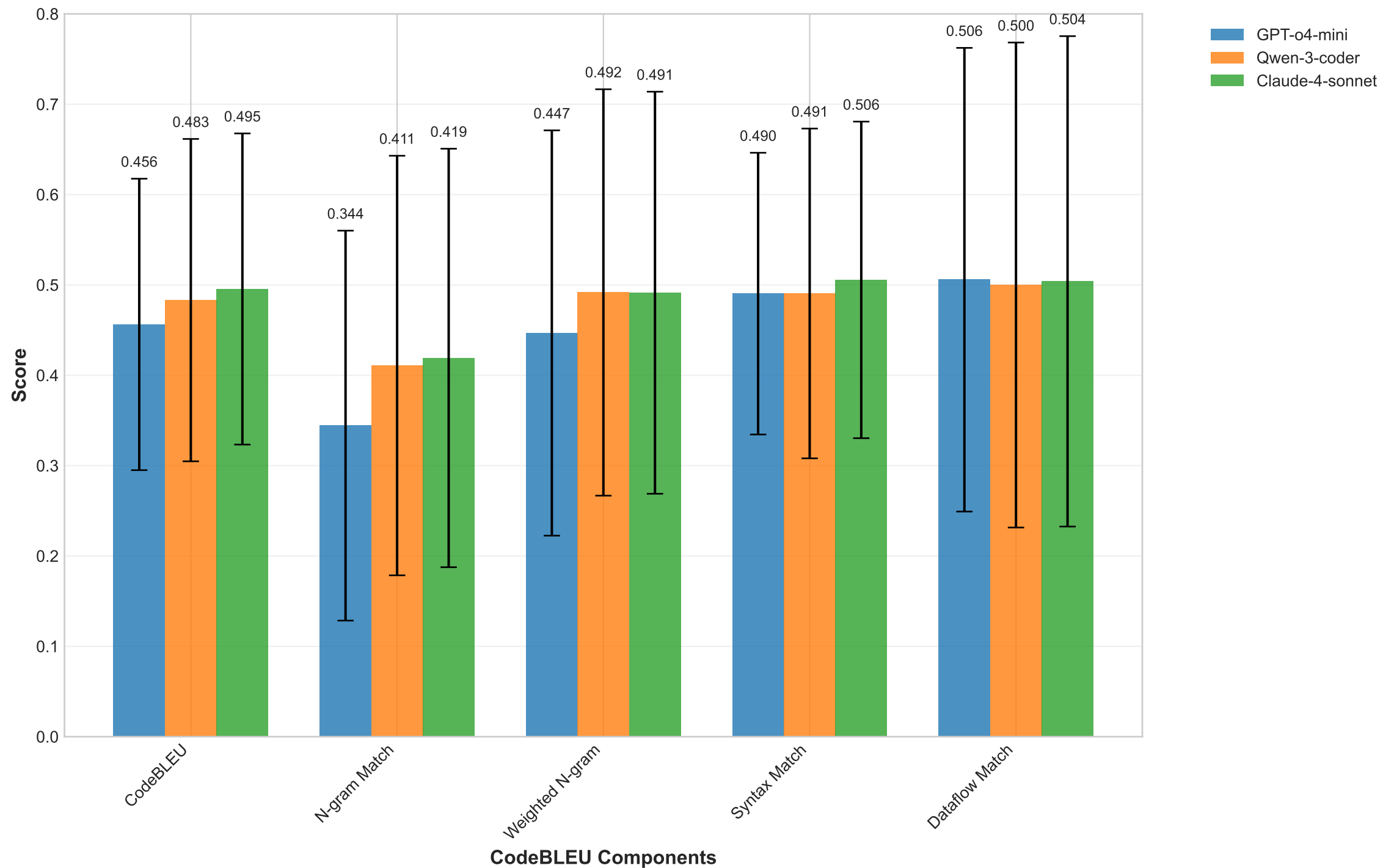
CodeBLEU Component Analysis for LLM-Generated Code
