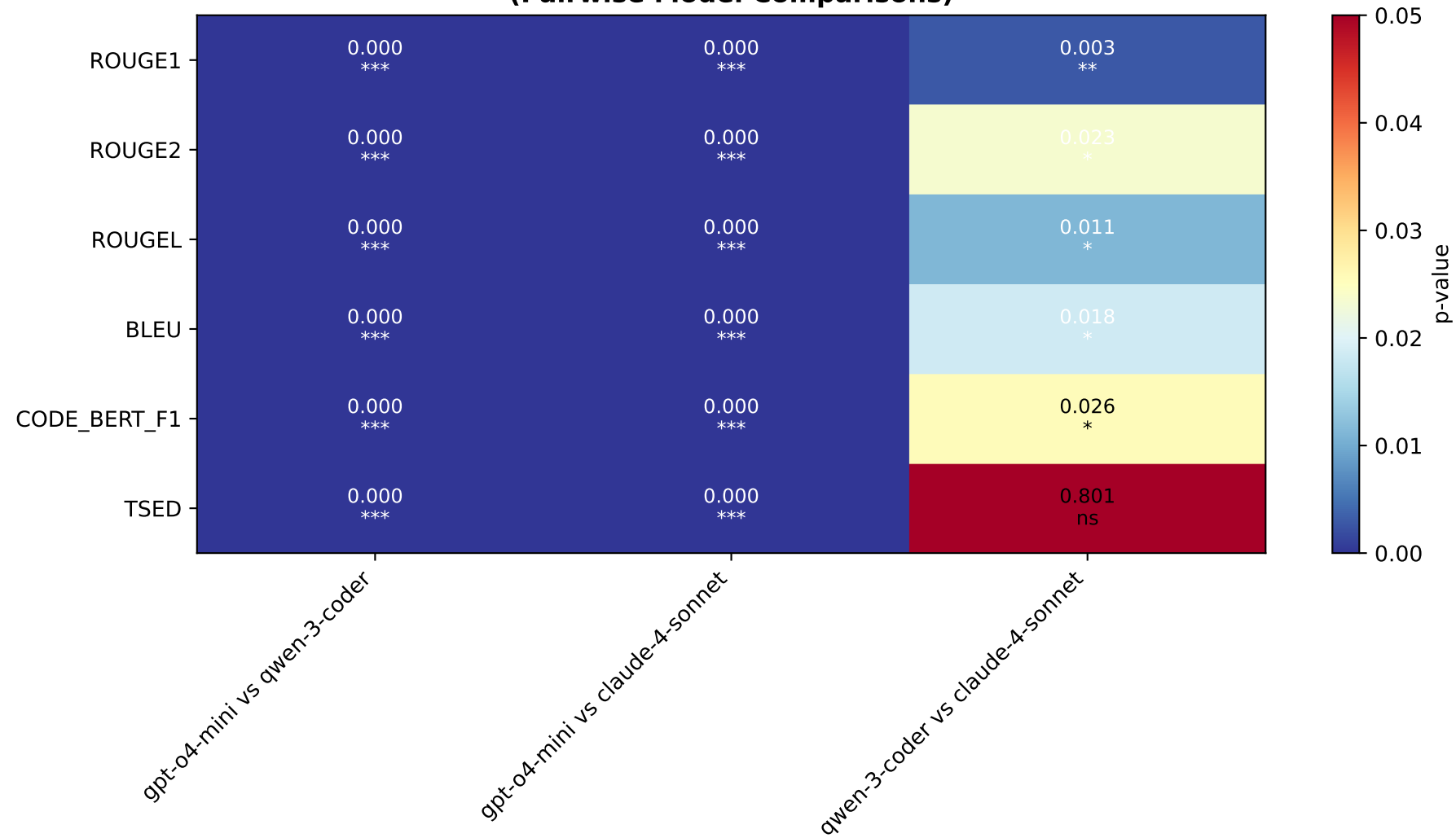
Statistical Significance Heatmap (Pairwise Model Comparisons)
