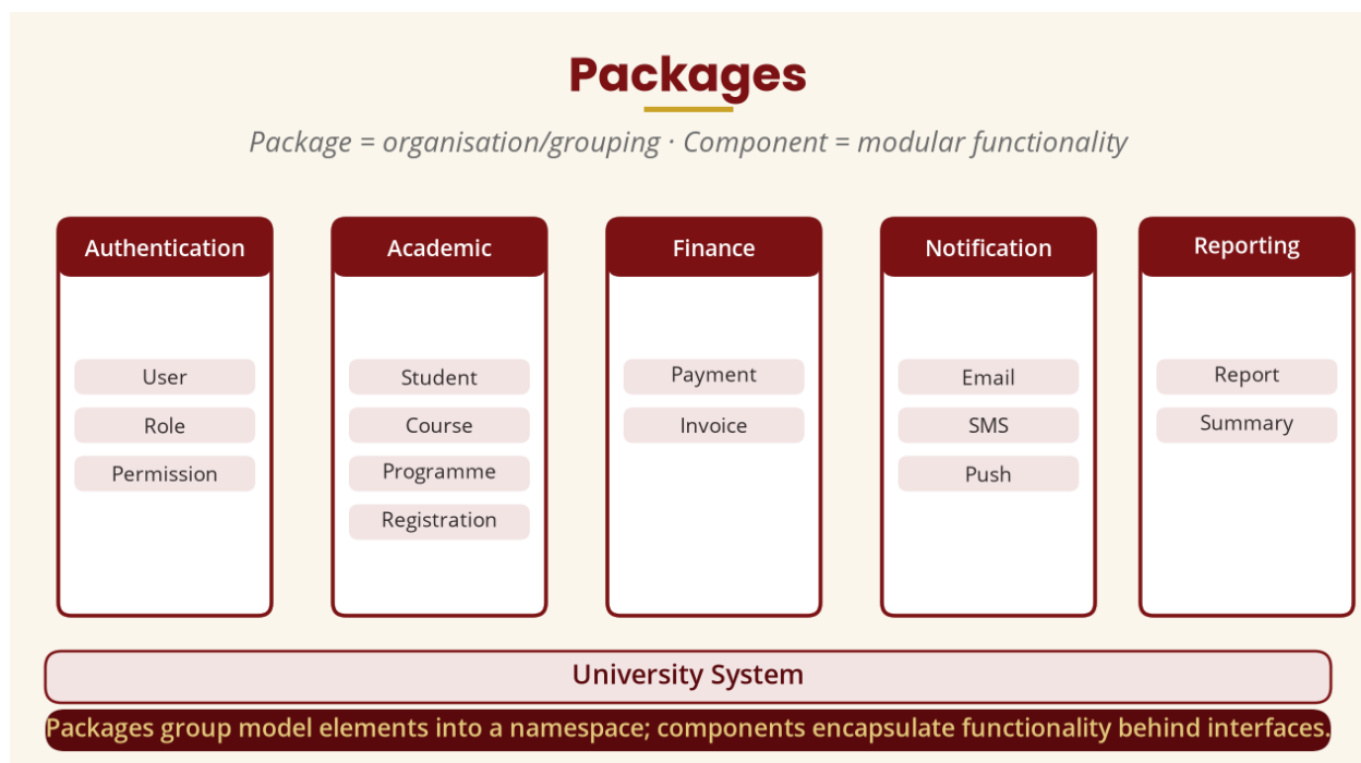
Figure 14 — Packages
