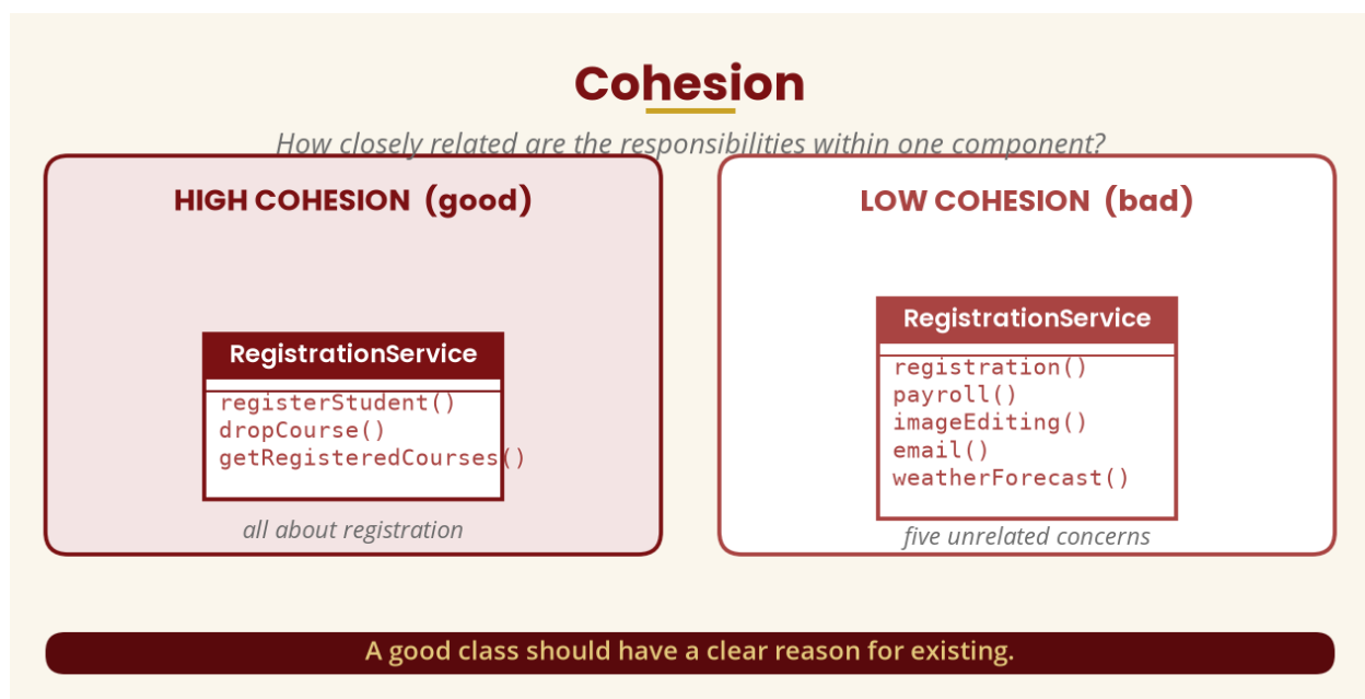
Figure 7 — Cohesion
