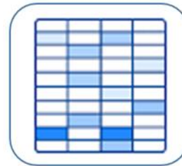
Wide-Column Store
