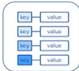
Key-Value Store
