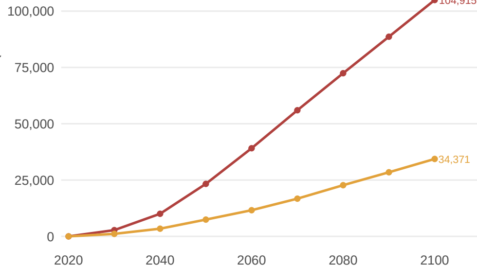
RCP 8.5 wet
