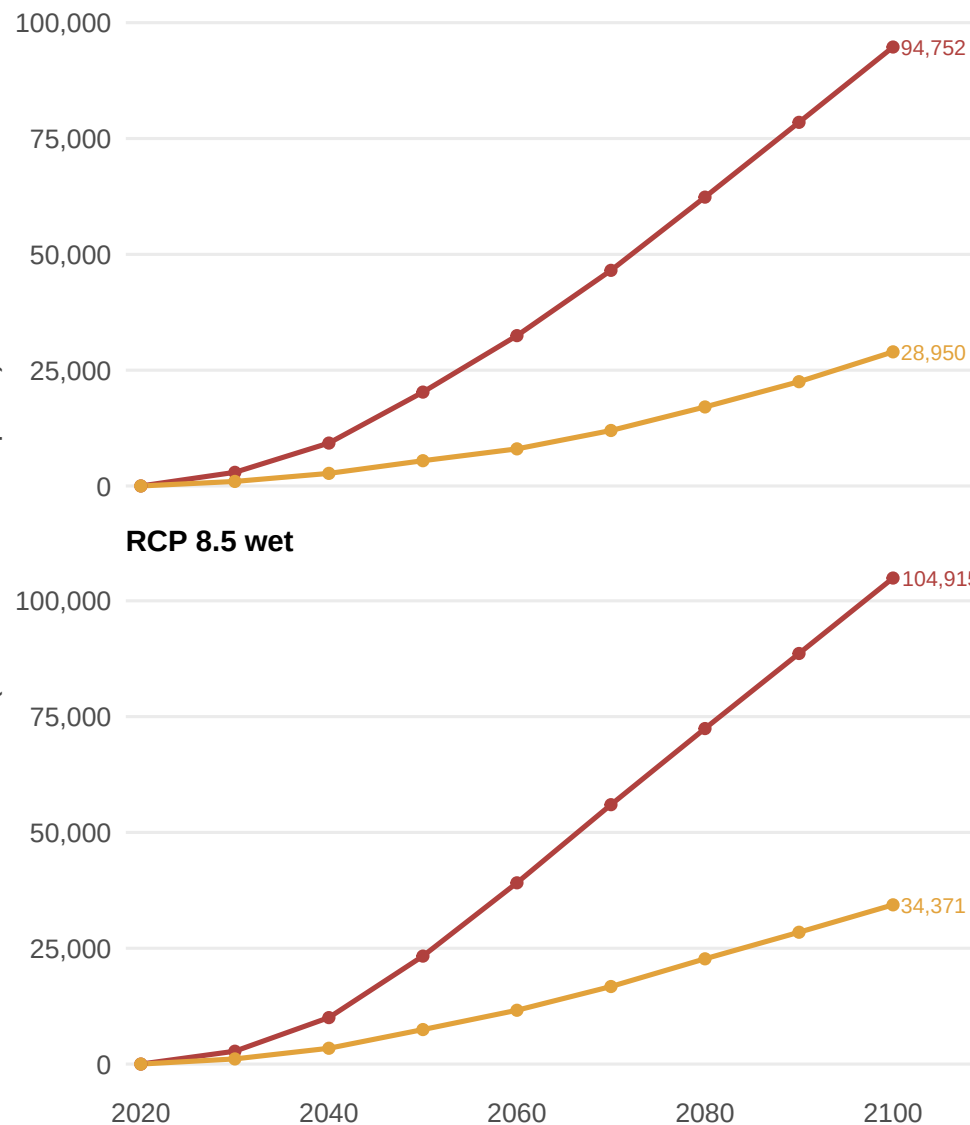
RCP 4.5 wet
