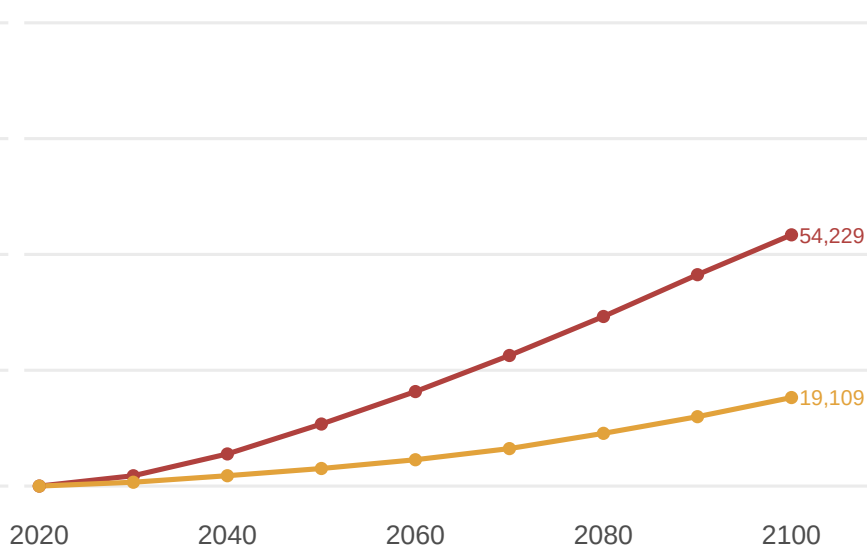
RCP 8.5 dry
