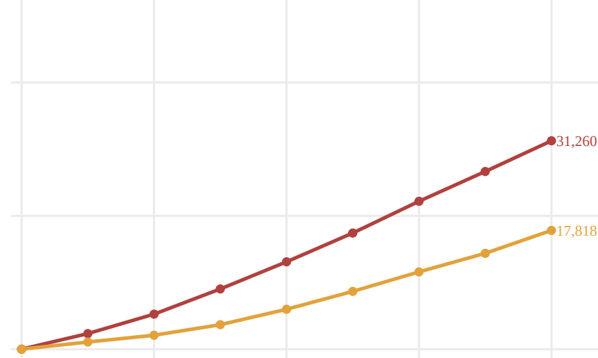
RCP 8.5 dry
