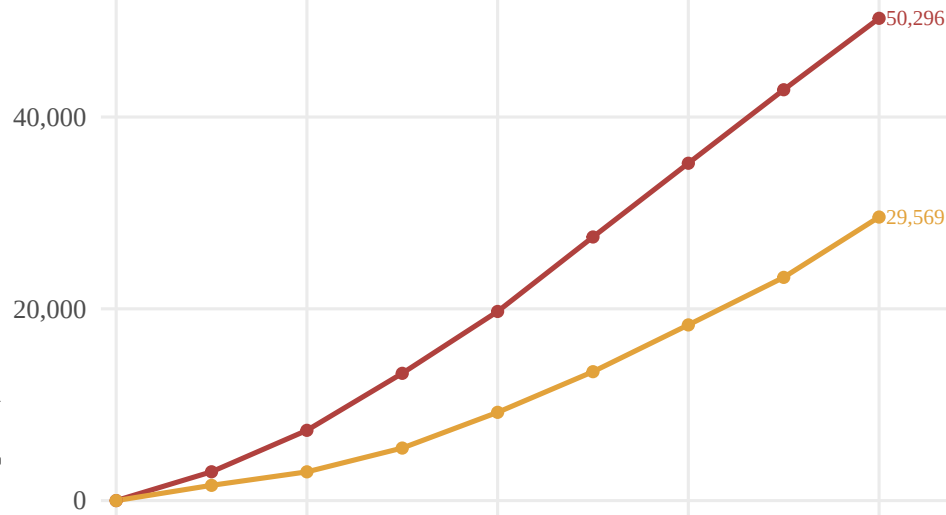
RCP 8.5 wet
