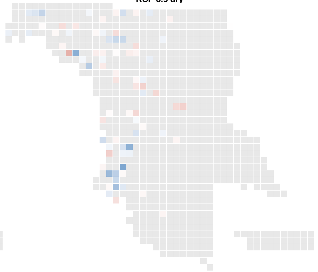
RCP 8.5 dry
