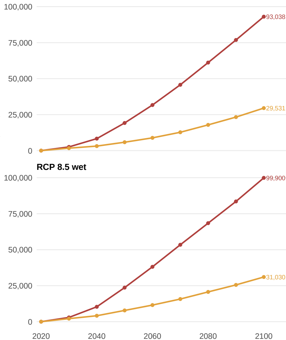
RCP 4.5 wet
