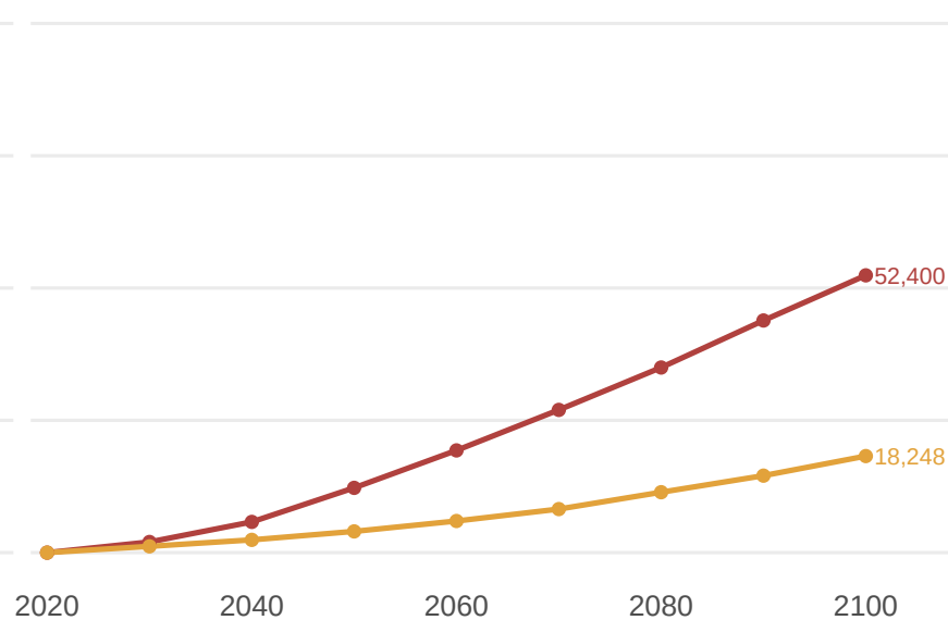
RCP 8.5 dry
