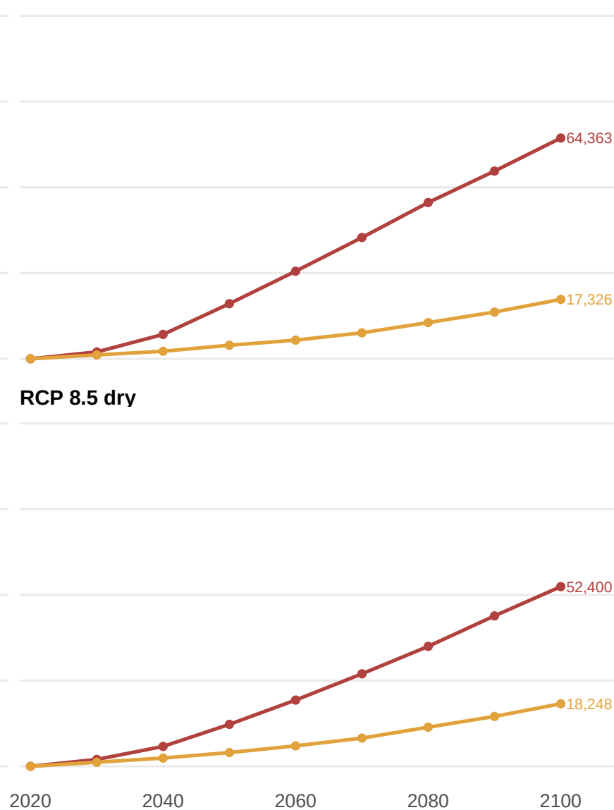
RCP 4.5 dry
