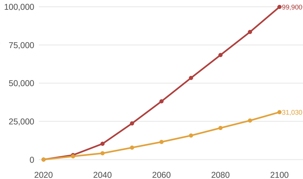
RCP 8.5 wet
