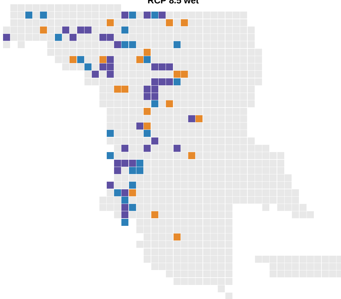
RCP 8.5 wet
