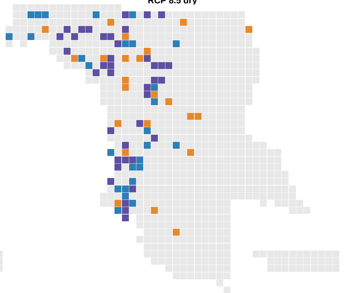
RCP 8.5 dry
