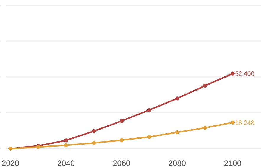
RCP 8.5 dry
