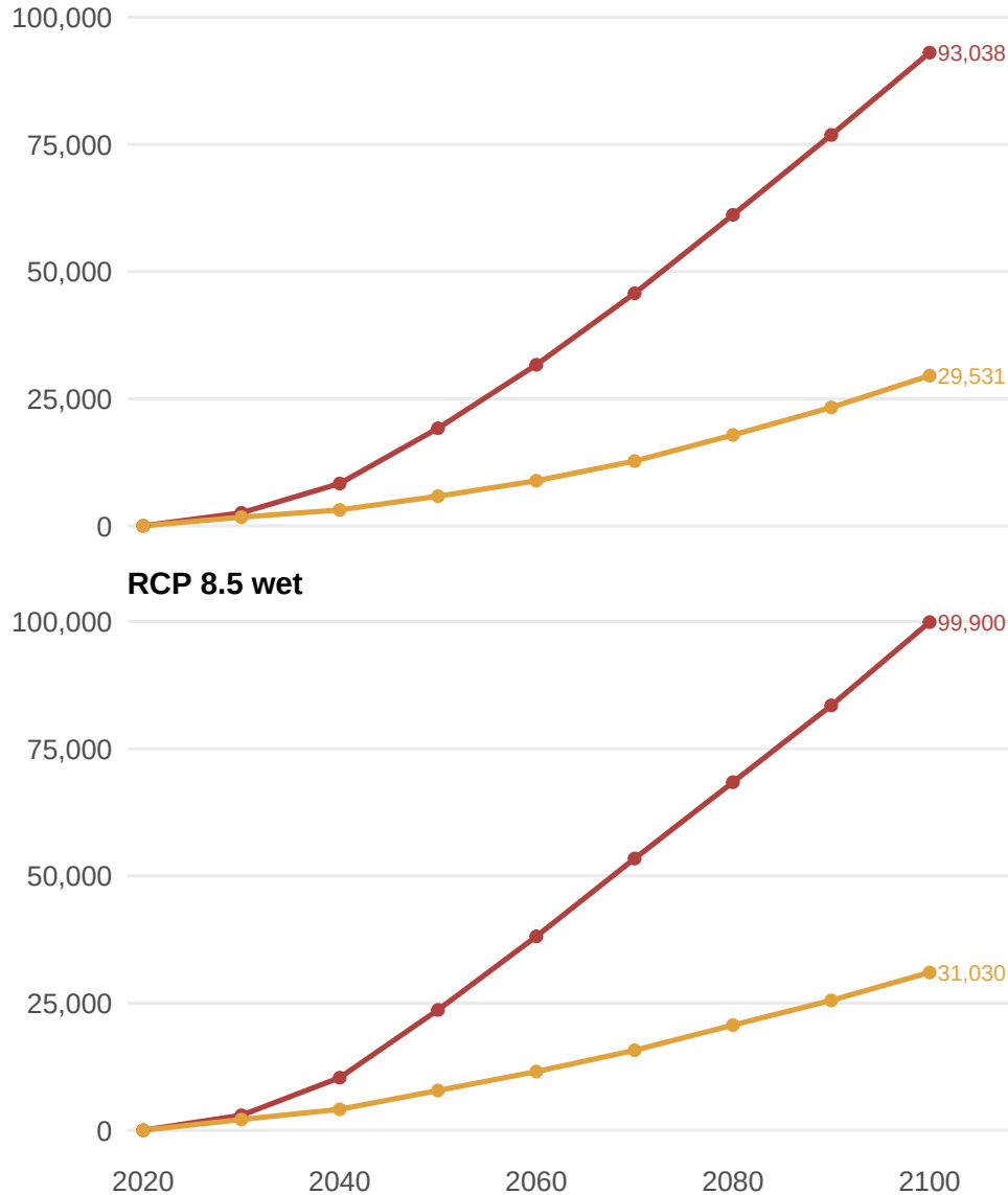
RCP 4.5 wet
