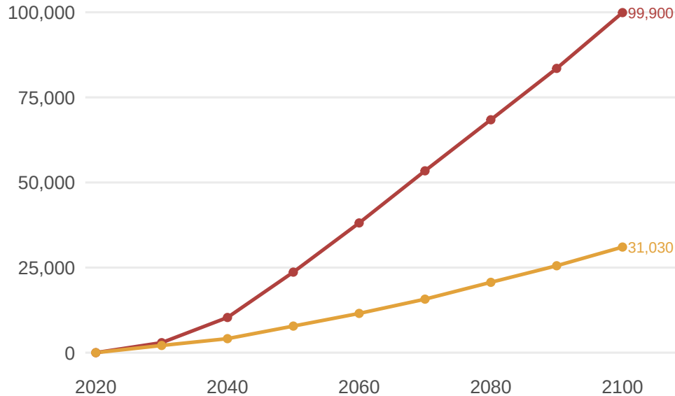
RCP 8.5 wet
