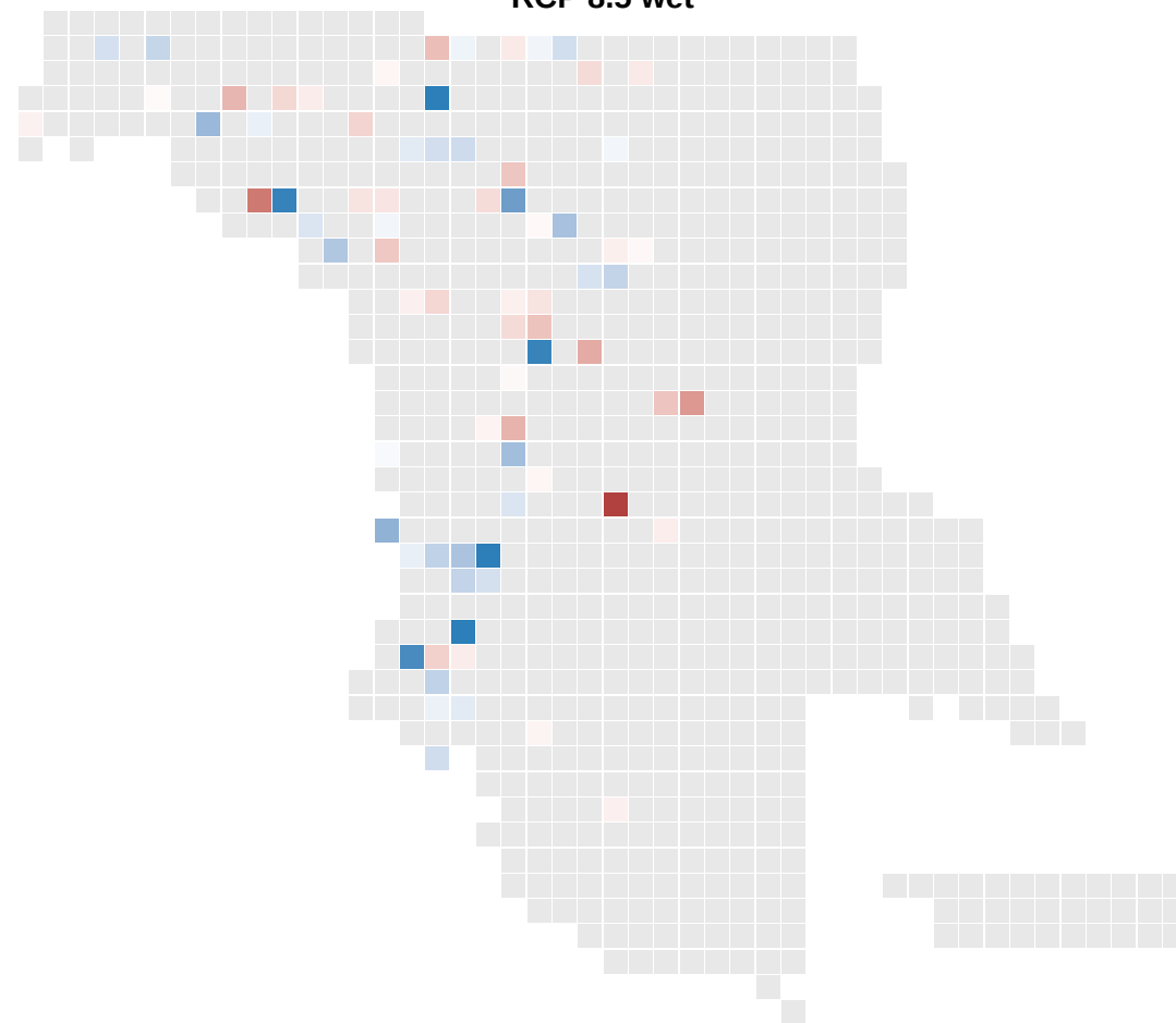
RCP 8.5 wet
