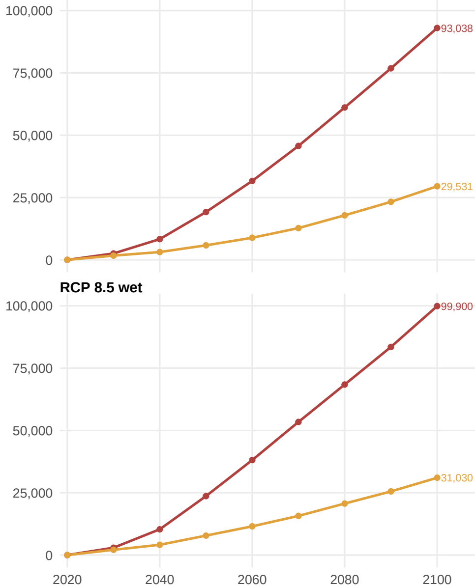
RCP 4.5 wet
