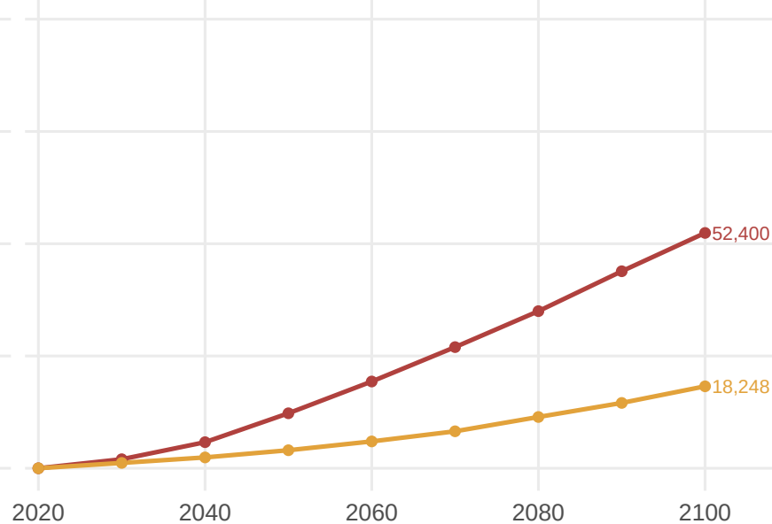
RCP 8.5 dry
