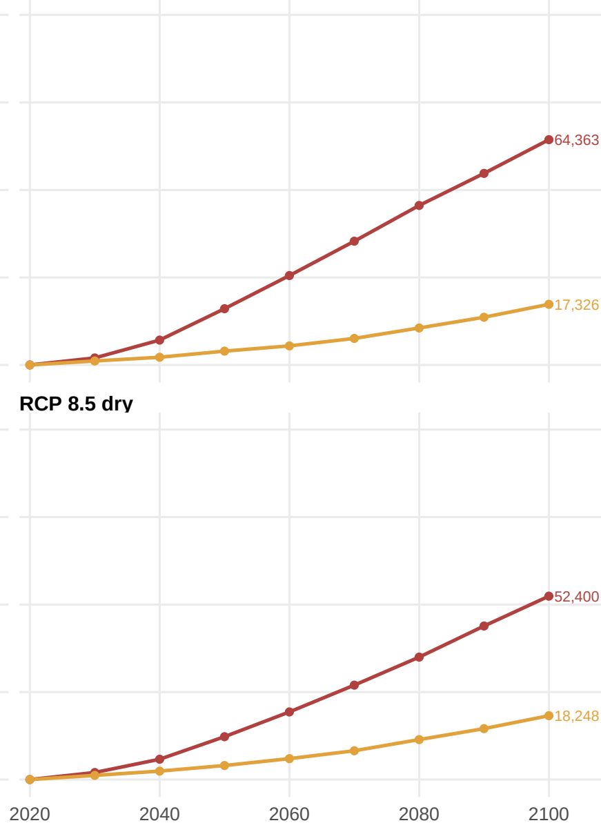
RCP 4.5 dry
