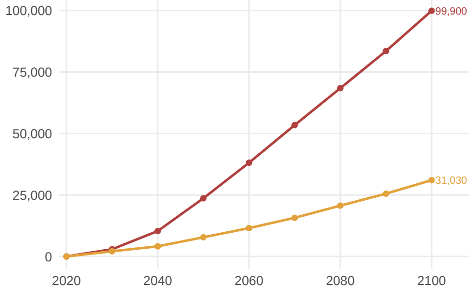
RCP 8.5 wet
