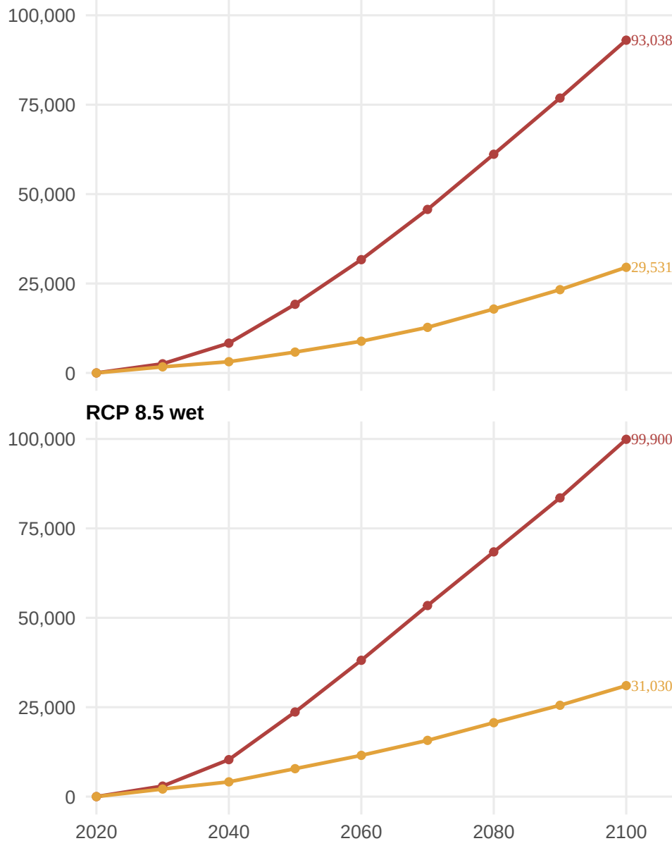
RCP 4.5 wet
