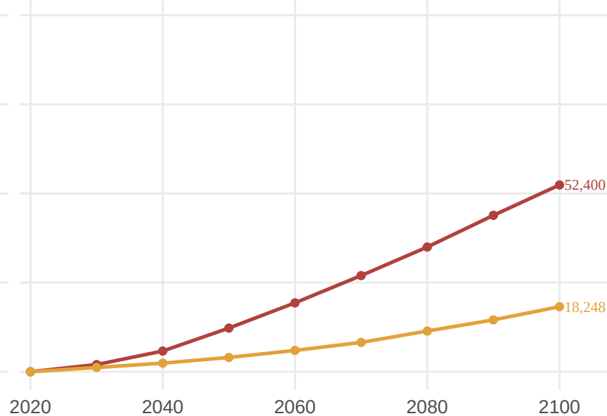
RCP 8.5 dry
