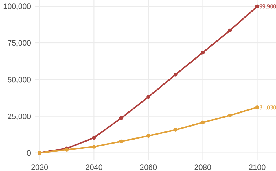
RCP 8.5 wet
