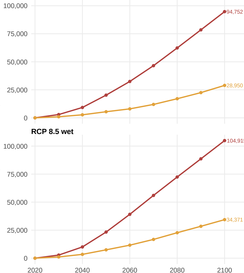
RCP 4.5 wet
