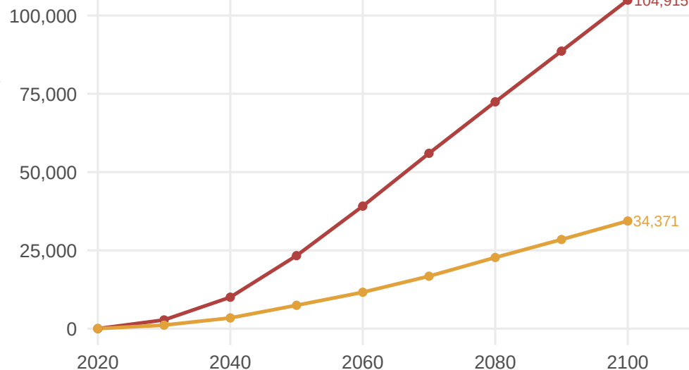
RCP 8.5 wet
