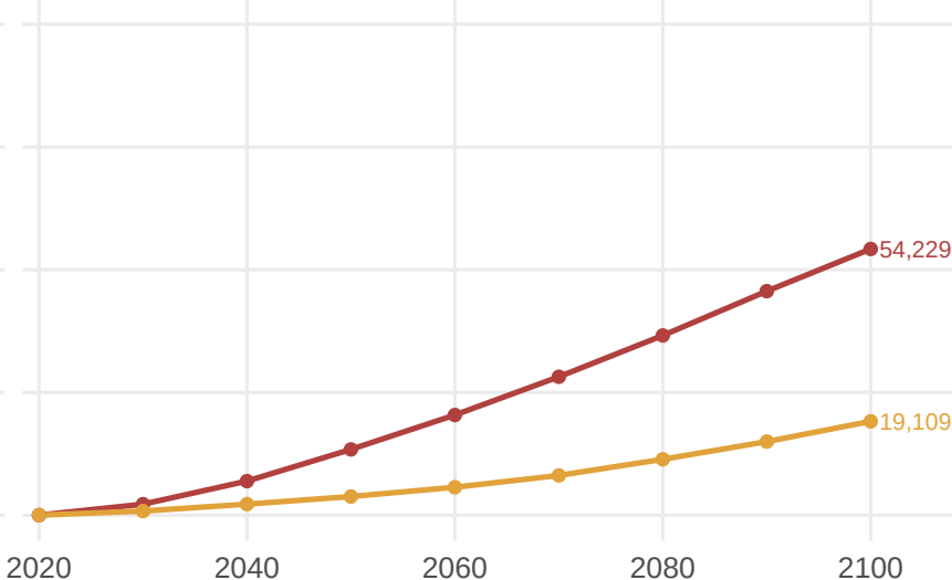
RCP 8.5 dry
