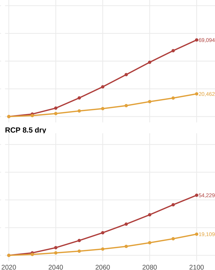
RCP 4.5 dry
