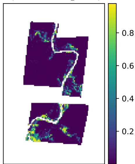
Physical OOF risk (R4_+forcing)
