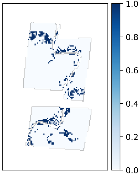
Labels (flooded cells)
