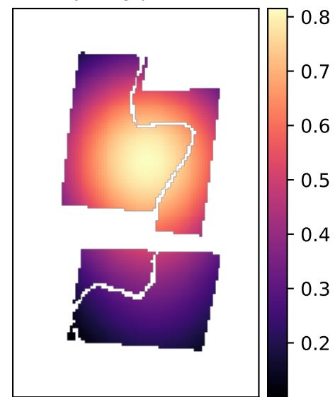
Social layer: log1p mentions/km 2
