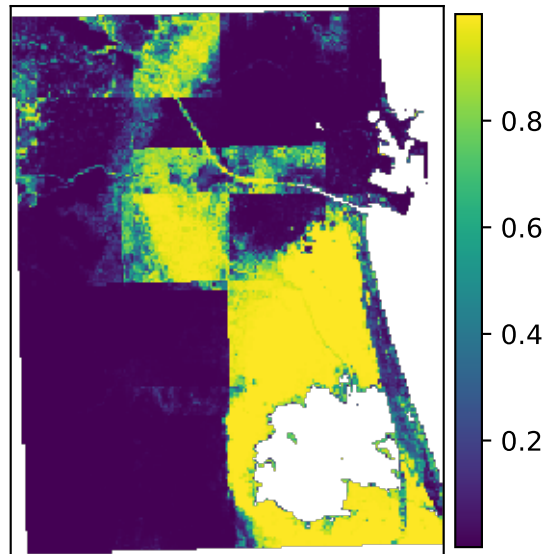
Physical OOF risk (R5_+sar_event)
