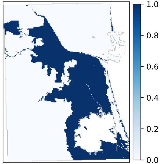
Labels (flooded cells)
