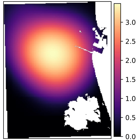
Social layer: log1p mentions/km 2
