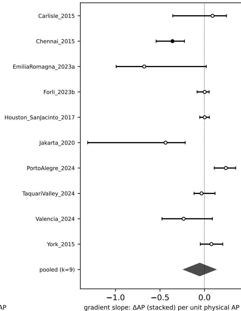
Saturation gradient per city (ordering A; filled = localisable social layer; pooled = tier A, all; 95% CIs)
