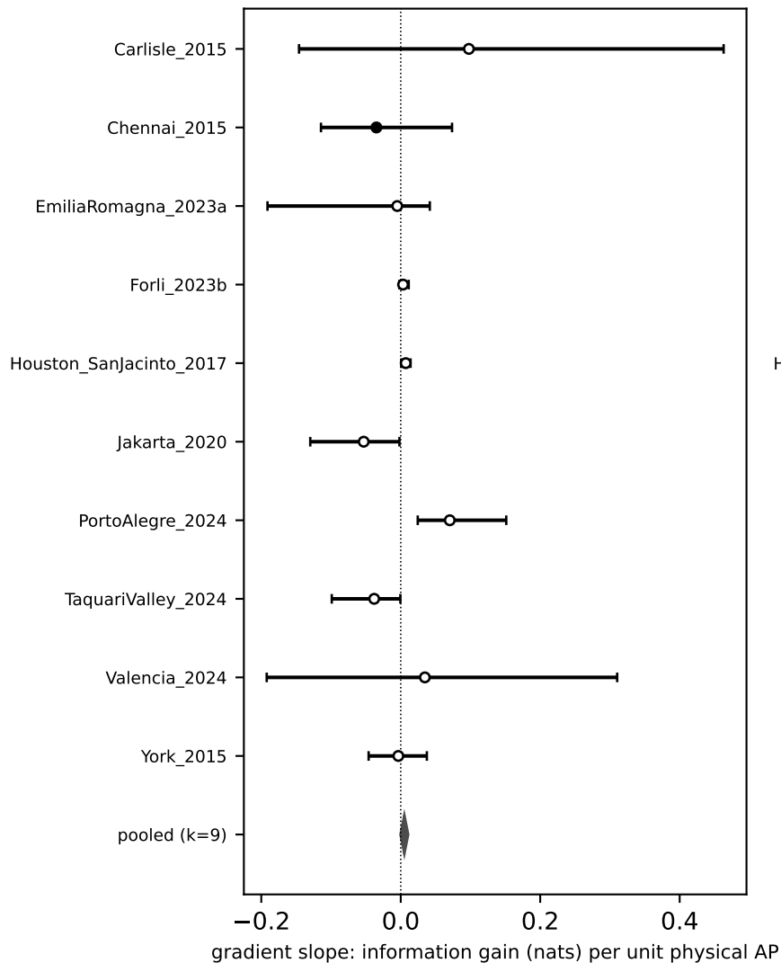
Saturation gradient per city (ordering A; filled = localisable social layer; pooled = tier A, all; 95% CIs)
