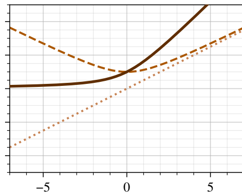
squareplus
