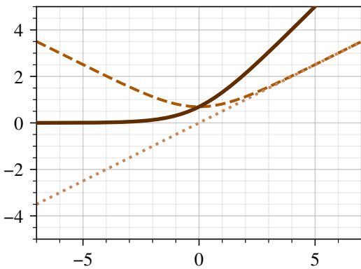
softplus
