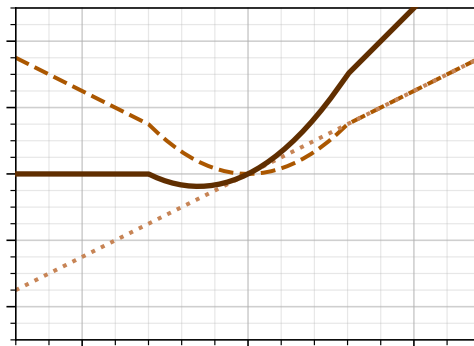
relu
