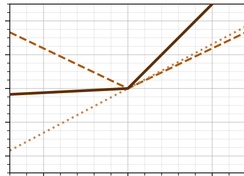
silu
