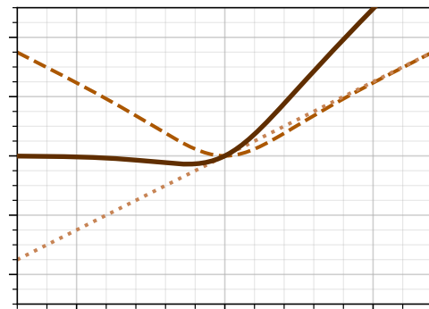
squareplus
