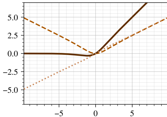
mish
