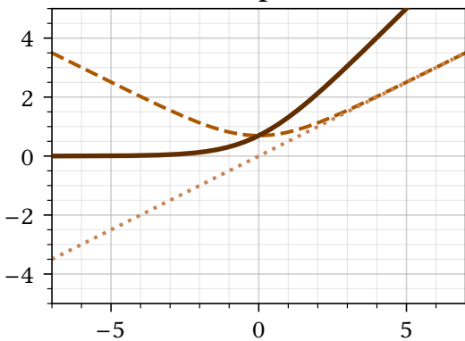
softplus
