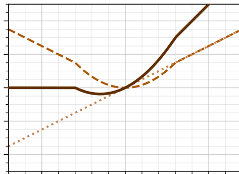
relu
