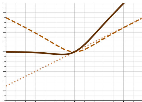
squareplus
