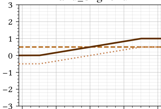
soft_sign
