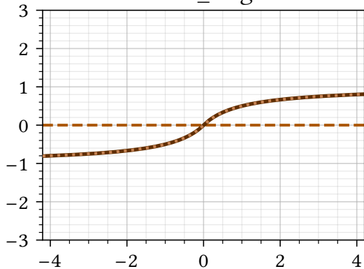
soft_sign
