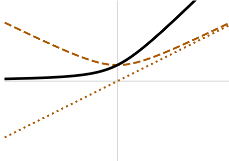
Squareplus
