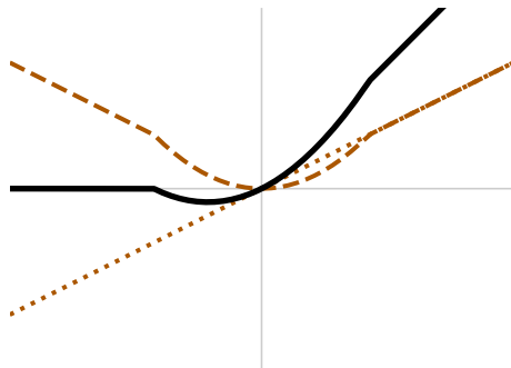
Hard SiLU
