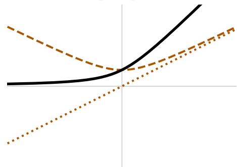
Squareplus
