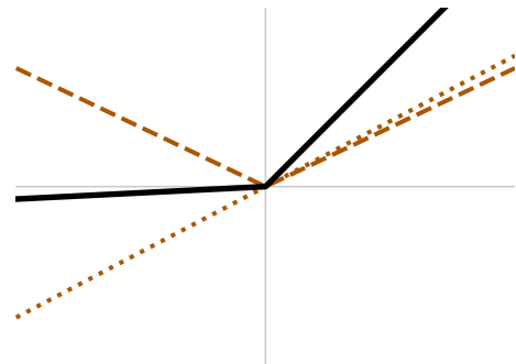
Leaky ReLU
