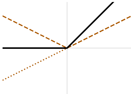
ReLU
