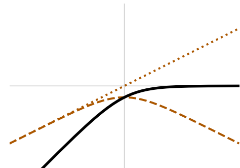
Log-sigmoid
