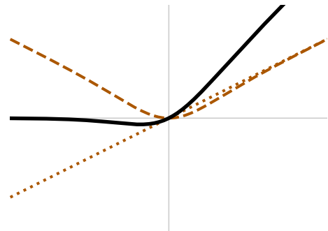
SiLU
