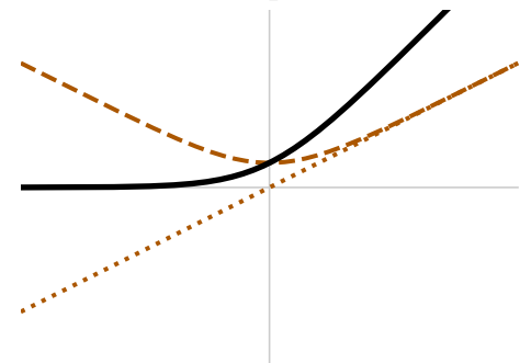
Softplus
