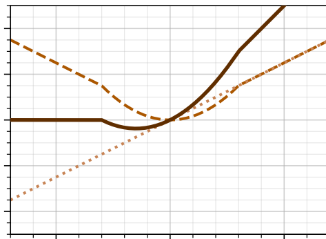
relu
