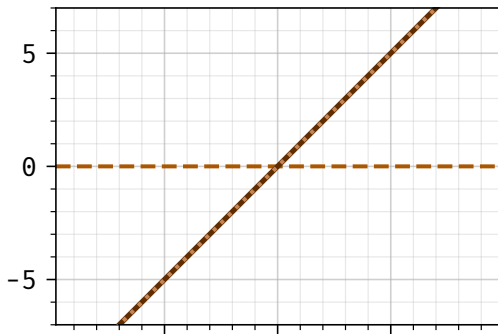
mish
