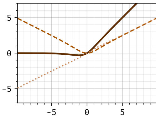
mish
