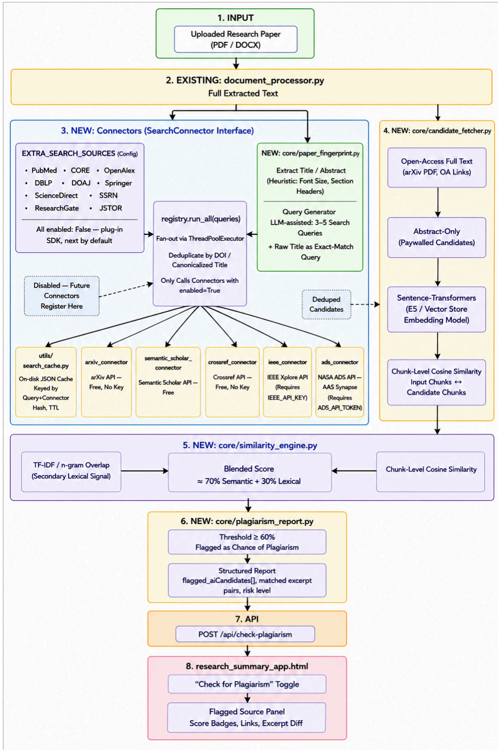
Fig. 1. Similarity Finder component architecture: fingerprinting, connector fan-out with on-disk caching, candidate content resolution, and blended-score reporting.
