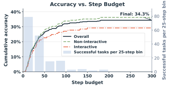
Figure 6: Cumulative accuracy of Kimi K2.6 under increasing step budgets. A task contributes to the accuracy at a given budget only if it is completed successfully within that number of steps.
