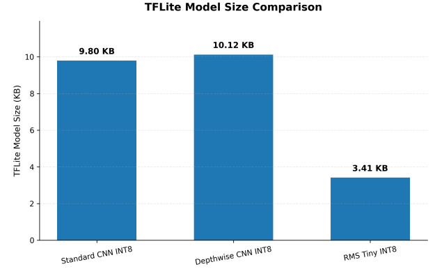
Figure 4: TFLite model size comparison for the three final INT8 deployment models.
