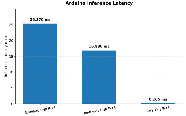
Figure 2: Measured neural-network inference latency on the Arduino Nano 33 BLE. The RMS Tiny INT8 result is also shown for context and is discussed later in the paper.
