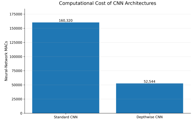
Figure 1: Neural-network computational cost of the Standard CNN and Depthwise CNN architectures. MAC counts exclude input preprocessing operations.
