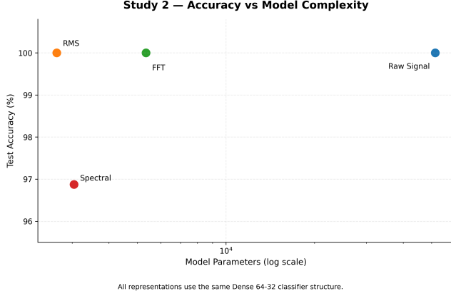
Figure 3: Test accuracy versus model complexity for the four controlled input representations. All models use the same Dense(64)-Dense(32)-Dense(4) classifier structure.
