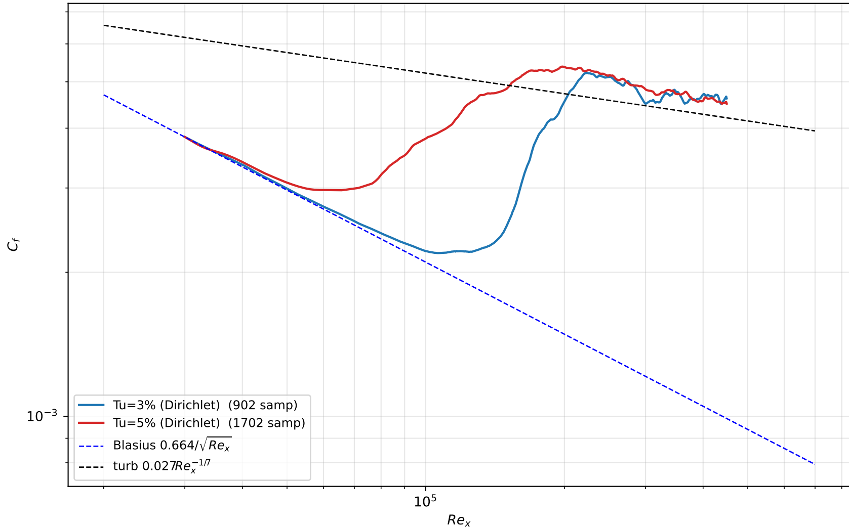
Skin friction: Tu=3\% vs Tu=5\% (both Dirichlet lid)
