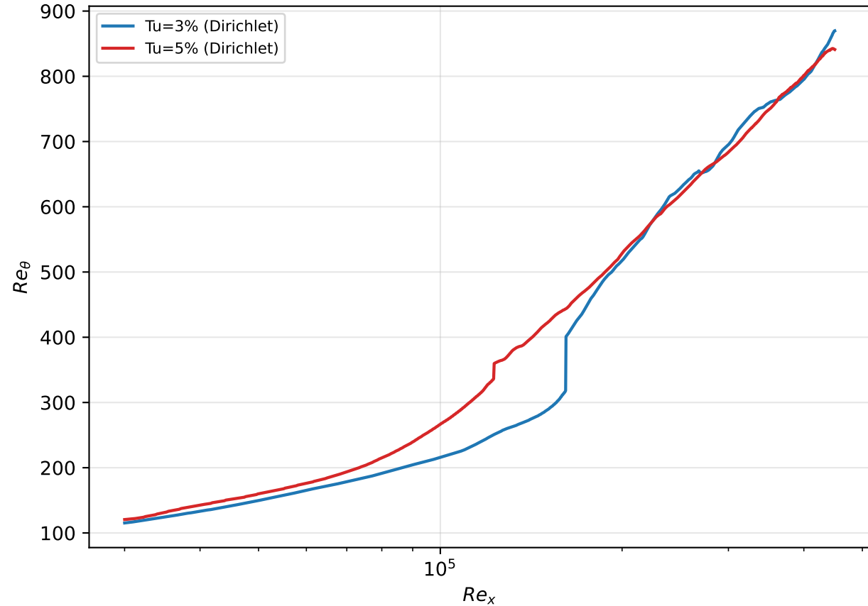
Momentum-thickness Reynolds number
