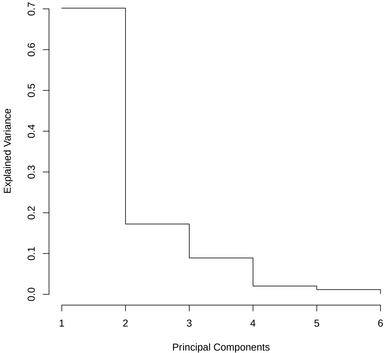
Scree Plot for DCA Year 2 PCA | Centered Only
