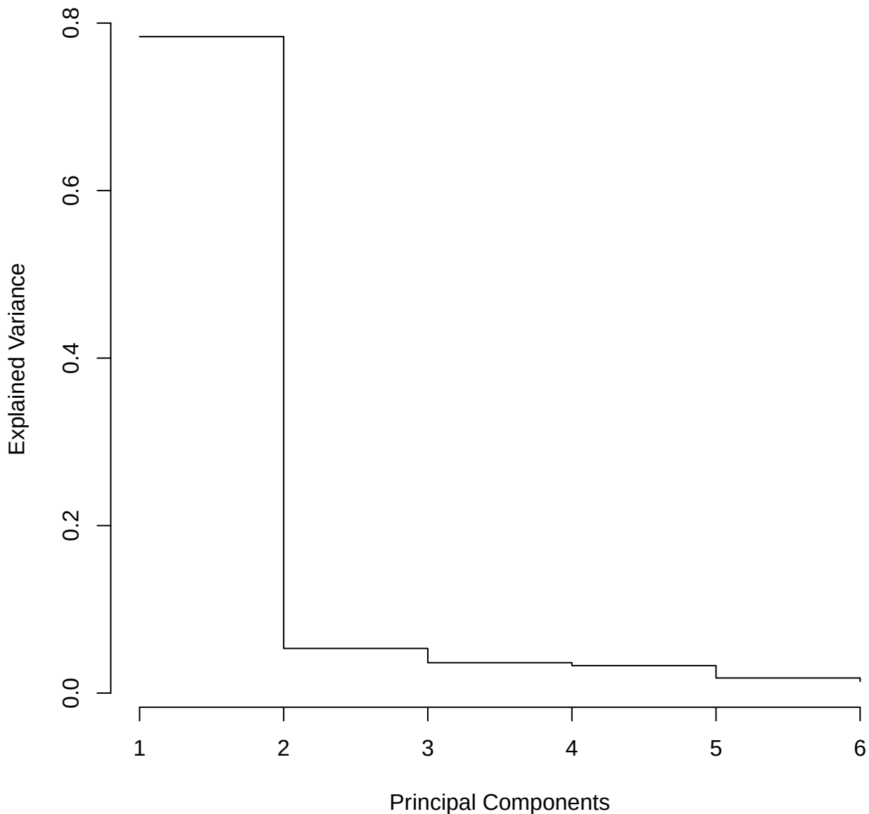
Scree Plot for DCA Year 1 PCA | Scaled Only
