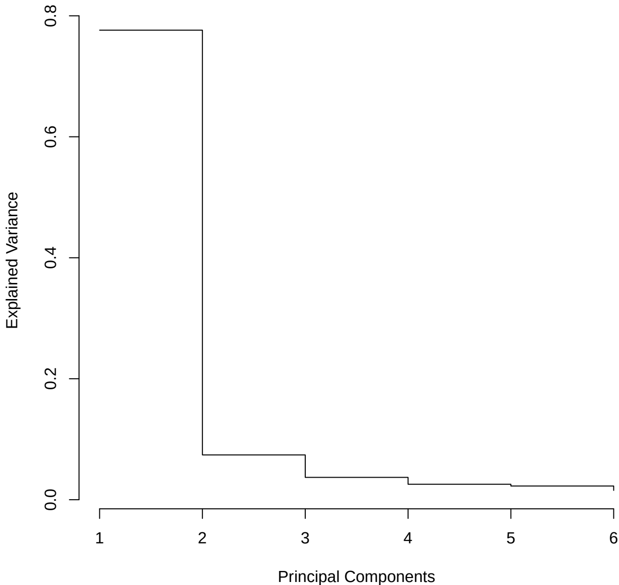
Scree Plot for DCA Year 2 PCA | Scaled Only
