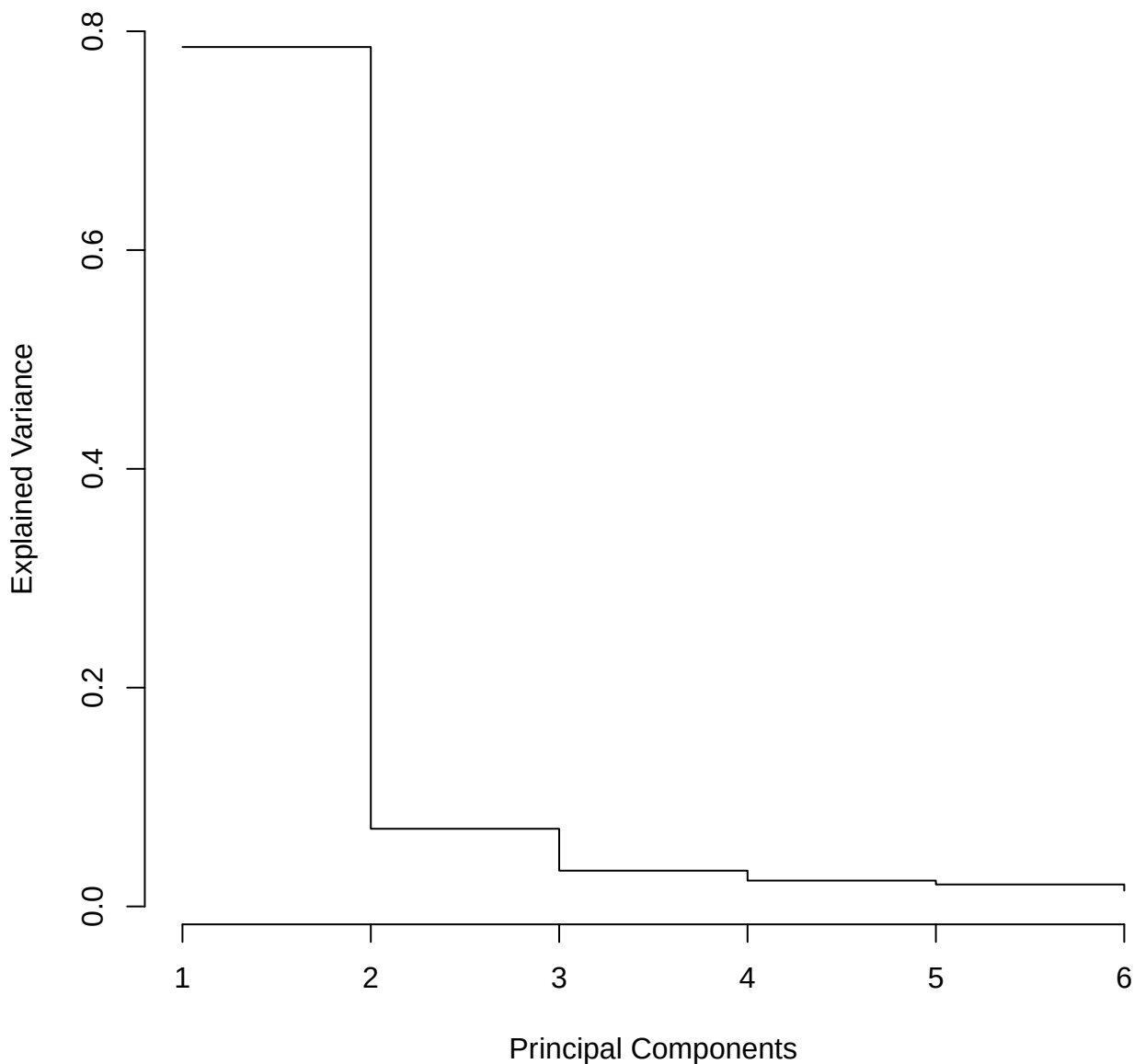
Scree Plot for CA Year 2 PCA | Scaled Only
