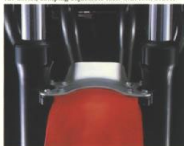
Air-assist, damping adjustable fork with fork brace.
